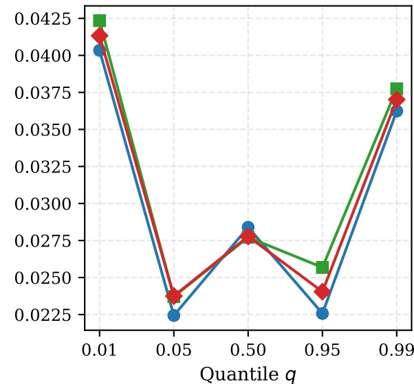
t (df=4)
