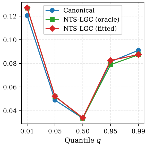
Gaussian
