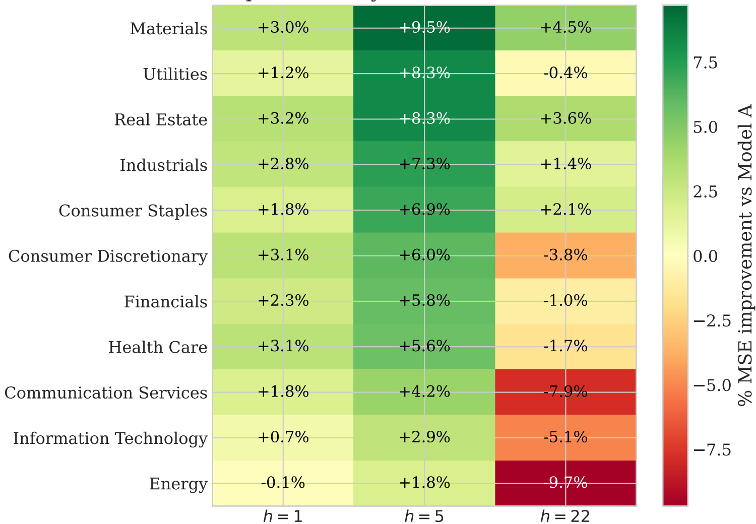
Model C improvement by GICS sector and forecast horizon
