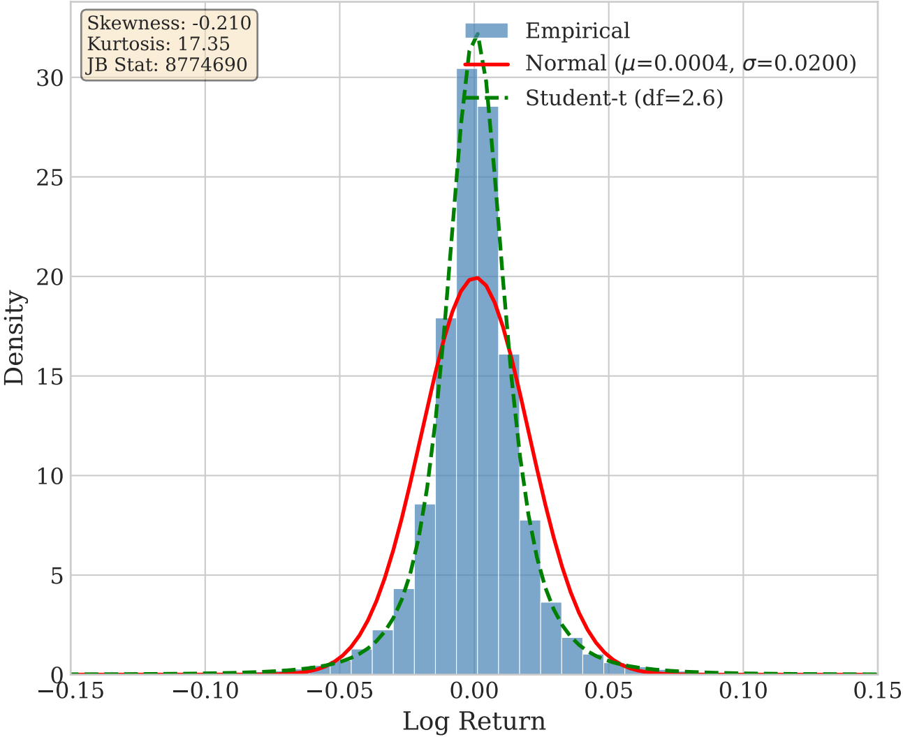
(a) Log-Return Distribution: Empirical vs Theoretical
