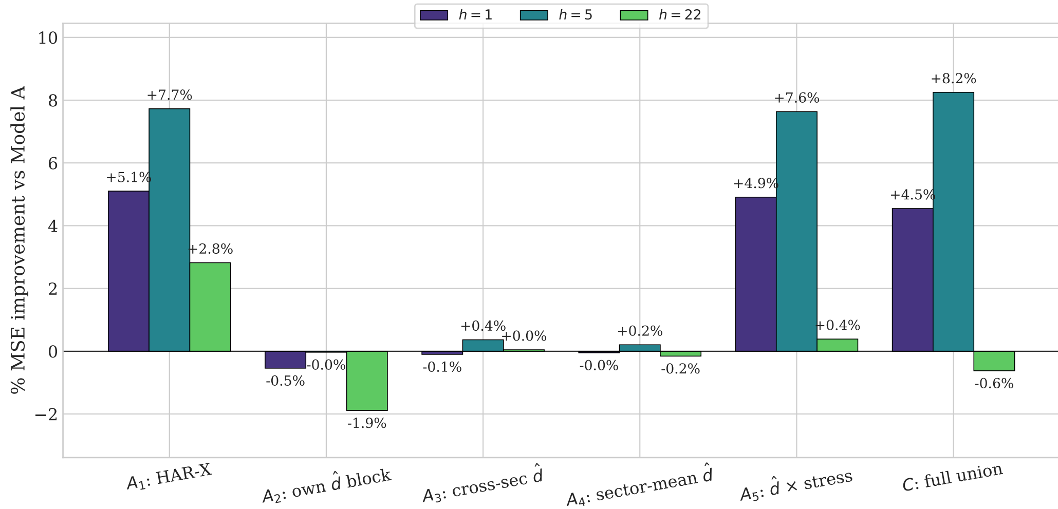
Layered ablation: each block's gain over the HAR baseline
