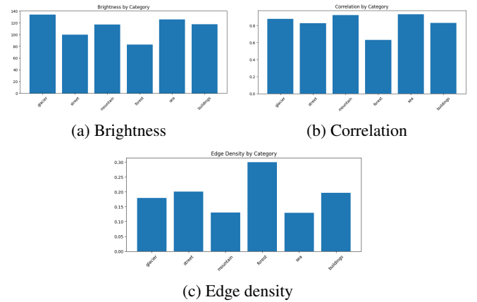
Fig. 7: Per-category statistical comparisons across the Intel dataset.
