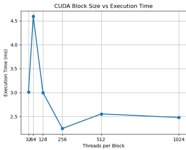
Figure 2: CUDA block size versus GPU execution time.
