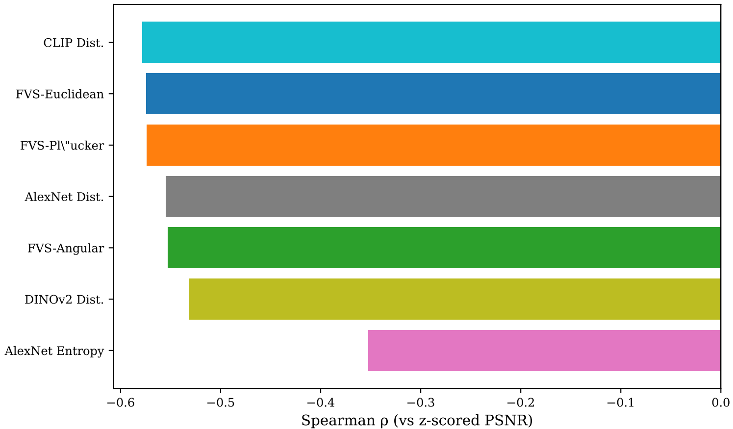
Correlations with z-scored PSNR
