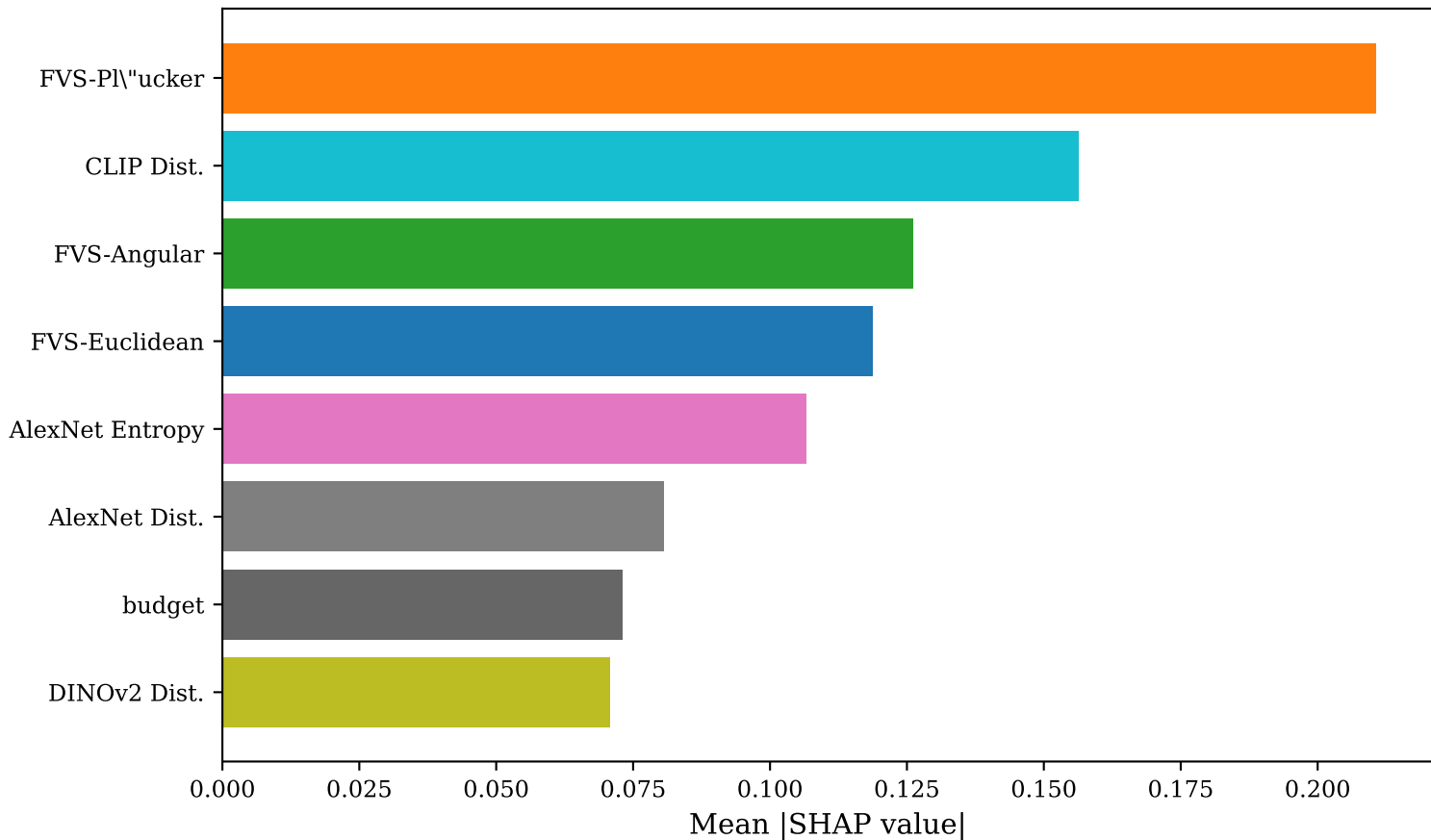
SHAP Feature Importance: z-scored PSNR
