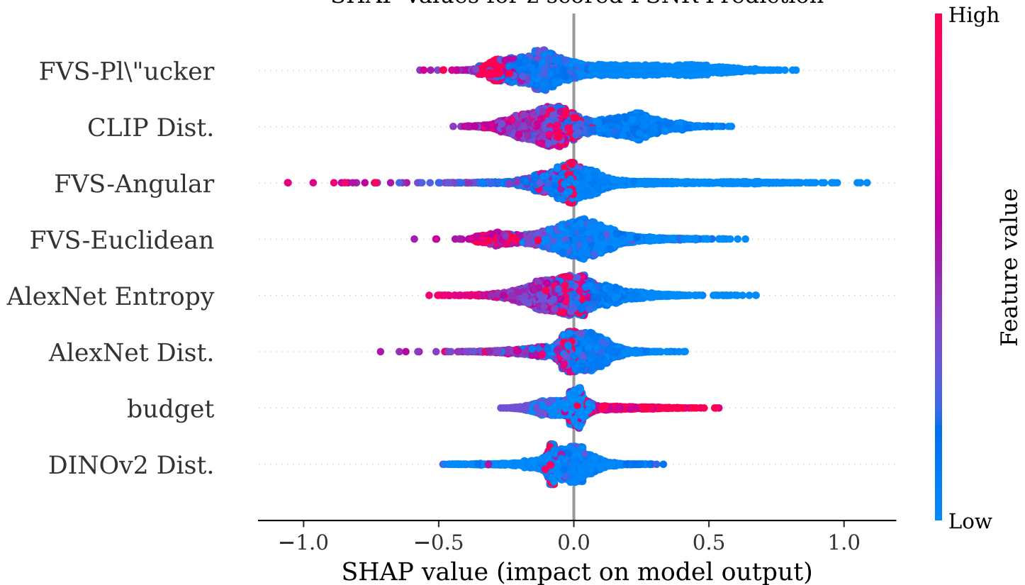
SHAP Values for z-scored PSNR Prediction
