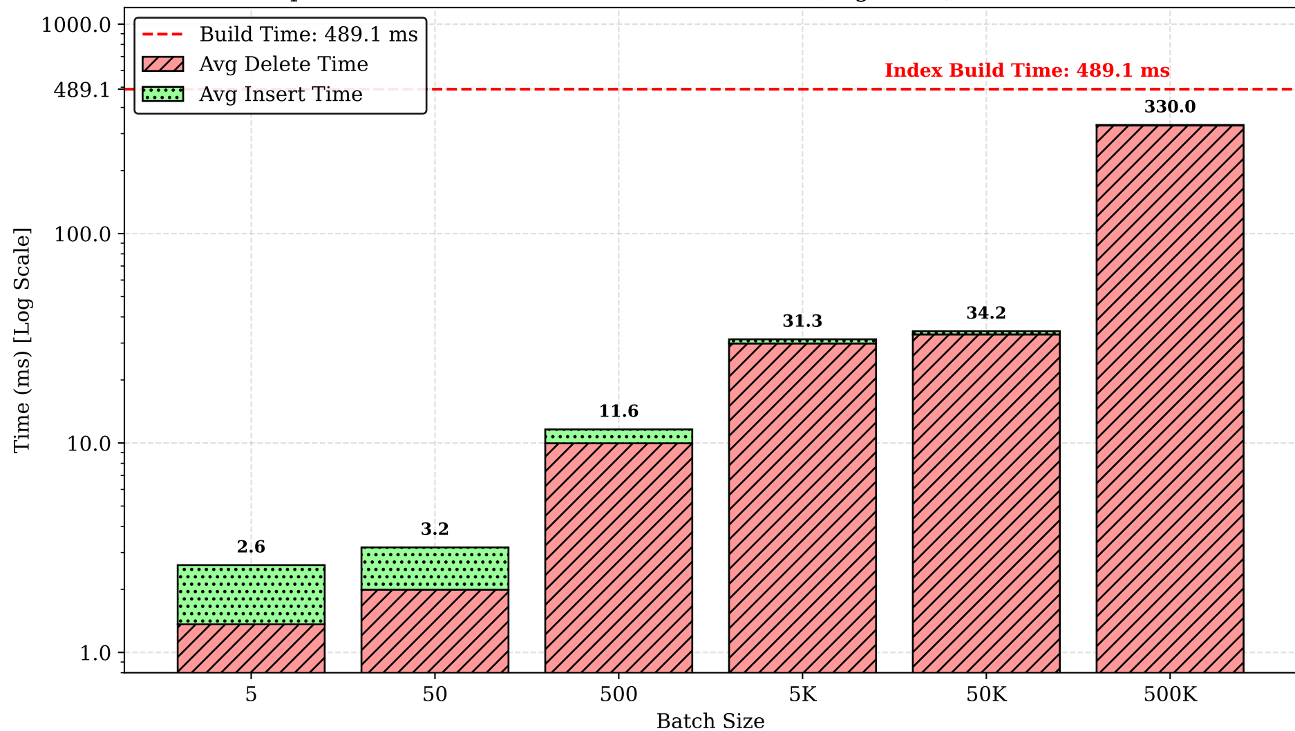
Update Performance: Delete vs Insert Time (Log Scale) [500M Normal]
