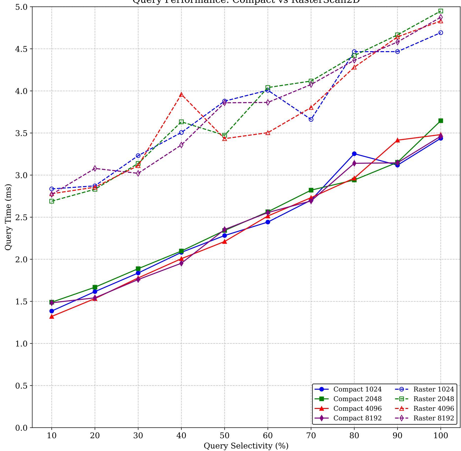
Query Performance: Compact vs RasterScan2D
