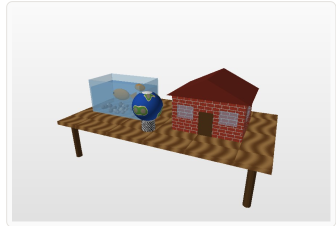
45_glass_and_textures.py
