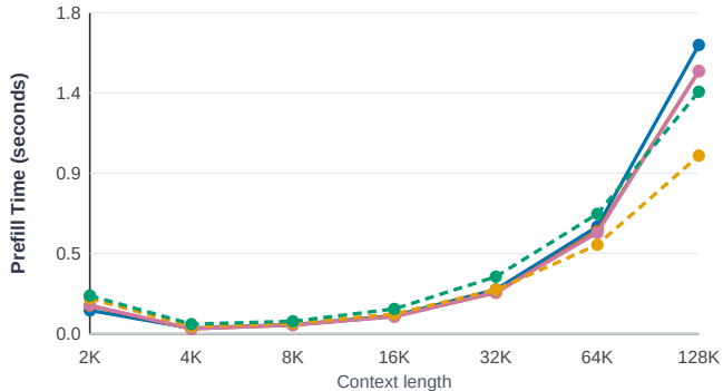
(a) Prefill Latency Scaling
