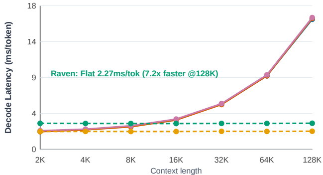
(b) Decode Latency Scaling
