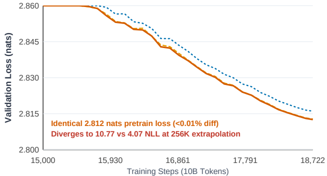
(b) Zoomed-In Resolution (Steps 15K-18.7K)
