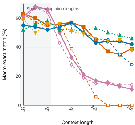
(b) BABILong
