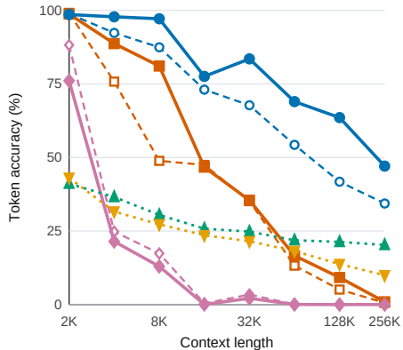
(a) Retrieval
