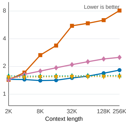
(c) Long-document
