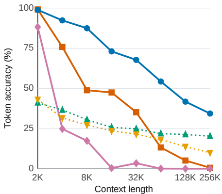
(a) Retrieval
