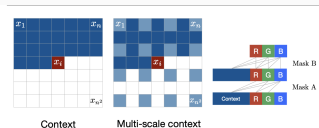
Figure 2. Left: To generate pixel x_i one conditions on all the previously generated pixels left and above of x_i . Center: To generate a pixel in the multi-scale case we can also condition on the subsampled image pixels (in light blue). Right: Diagram of the connectivity inside a masked convolution. In the first layer, each of the RGB channels is connected to previous channels and to the context, but is not connected to itself. In subsequent layers, the channels are also connected to themselves.
