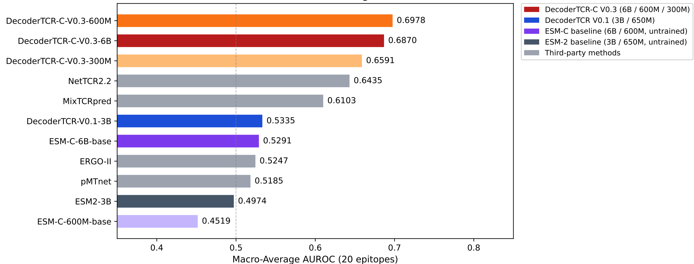
IMMREP2023: macro-average AUROC
