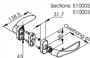
1862 FLOW paired lever handles 8 mm square spindle Zamak, polyamide base
