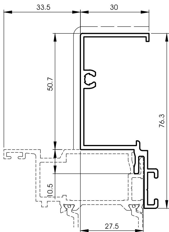
420082 Offset reveal liner 120 mm
