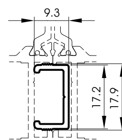
420066 Static joining piece for large chamber
