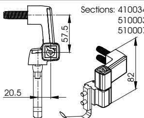
A5084 Corner hinge Aluminium
