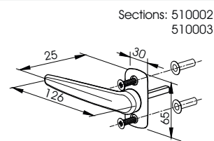
1870 HORUS extra-flat handle 8 mm square spindle Zamak
