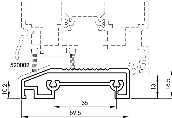
520008 Standard sill
