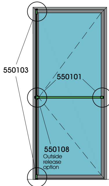
2 or 3 points top and bottom
