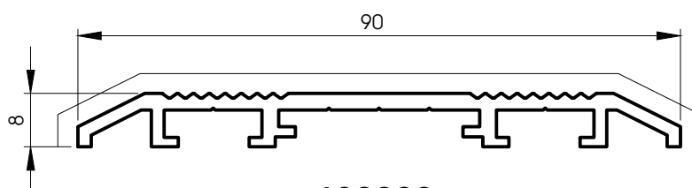
620000 90 x 8 Threshold
