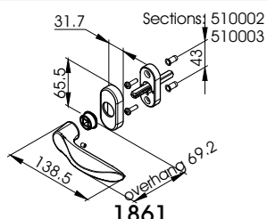
1861 FLOW paired lever handles 8 mm square spindle Zamak, polyamide base
