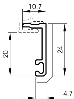
420005 24 mm architrave
