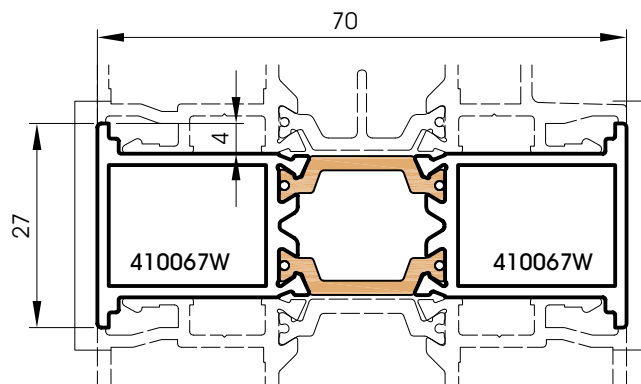
410067 180° joining piece
