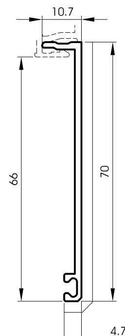
420004 70 mm architrave
