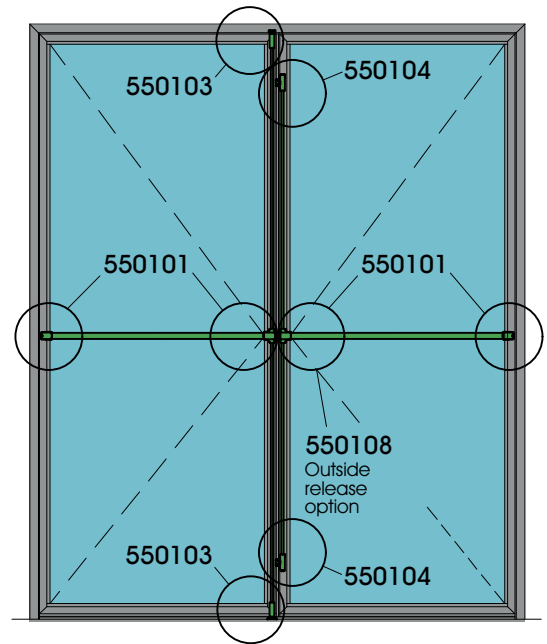
2 points top and bottom secondary leaf
