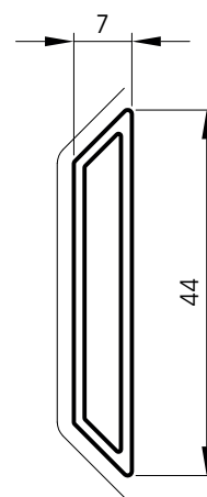
420062 "Petit bois" decorative strip
