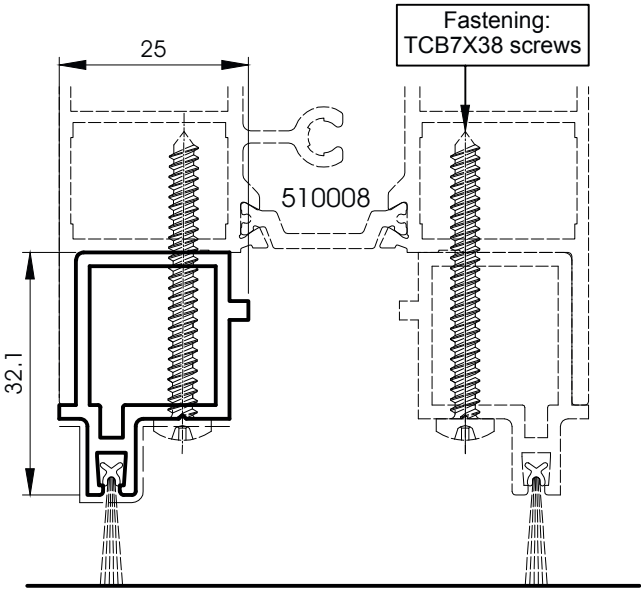
520013 Brush seal section for kick-plate ref. 510008
