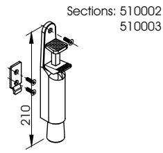
1817 Push-down stopper Locking stroke 30 mm Aluminium
