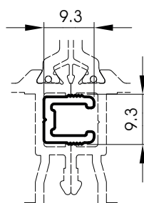
420003 Static joining piece
