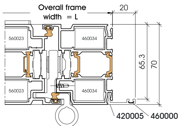
Architrave 420005
