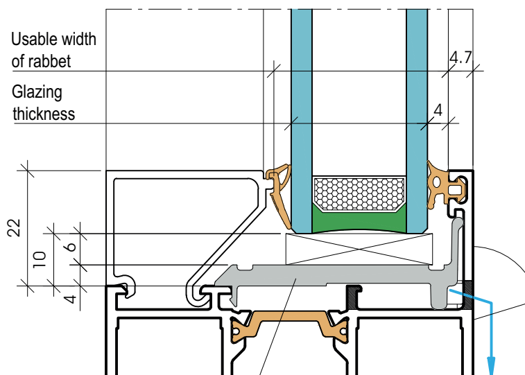
Glazing packer support 560001
