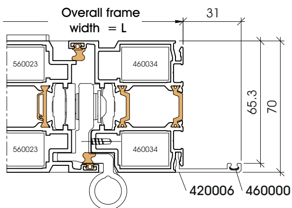
Architrave 420006
