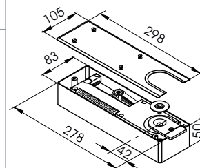
5661 Floor spring + cover plate Plate: polished stainless steel
