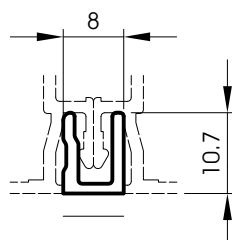
420002 Snap-in groove joining piece
