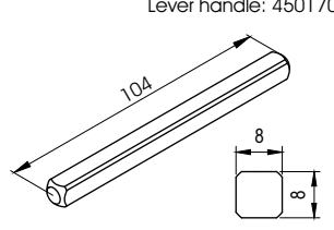
1894 Square spindle L=104mm Galv. steel
