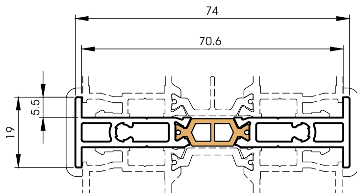
510029 Joining section
