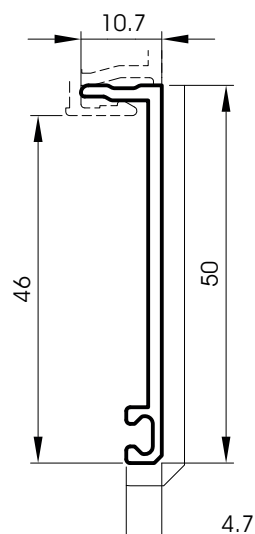
420028 50 mm architrave
