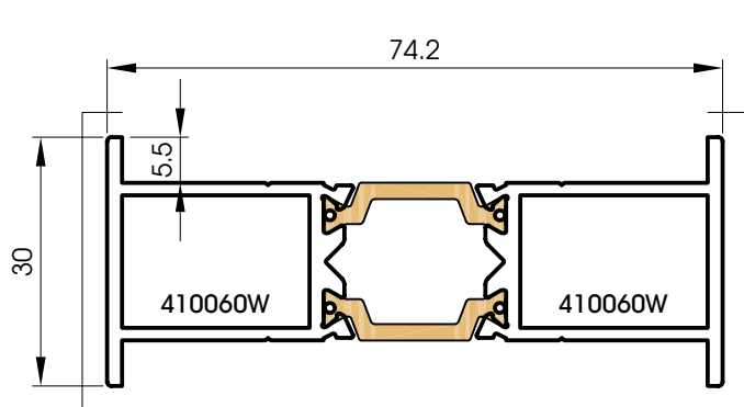
410060 180° joining piece
