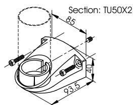
1637 Ø 50 mm tubular handle attachment Powder-coated aluminium
