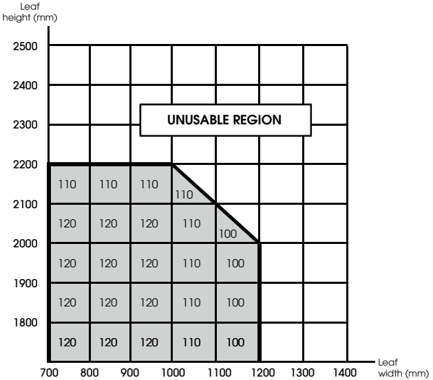
SURFACE-MOUNTING HINGES ref A5080
