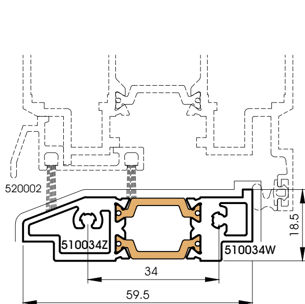
510034 Sill with thermal break
