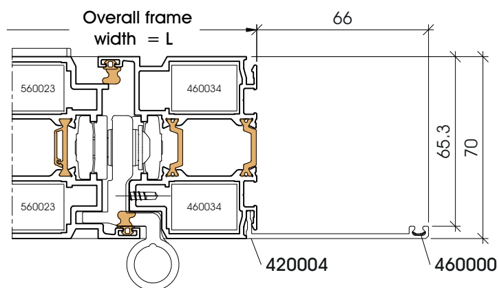
Architrave 420004
