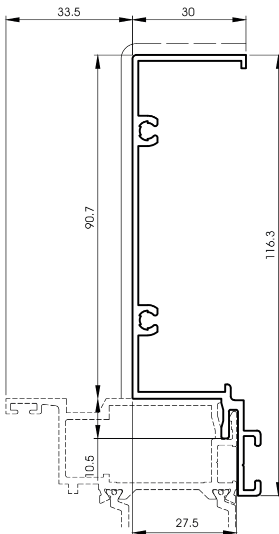
420084 Offset reveal liner 160 mm
