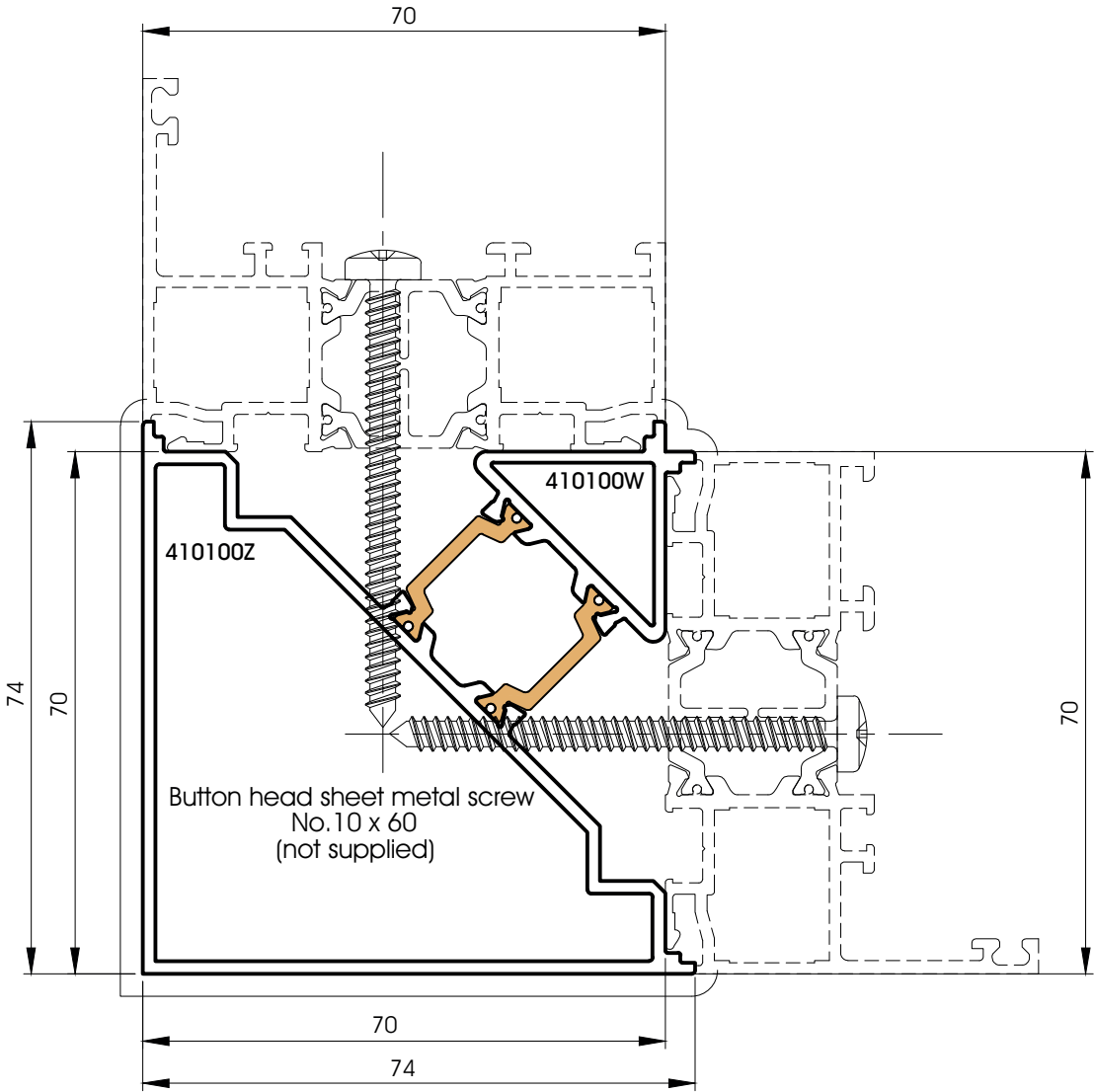
410100 90° out-facing post, 74mm
