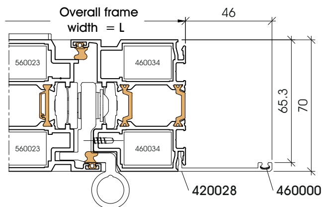
Architrave 420028
