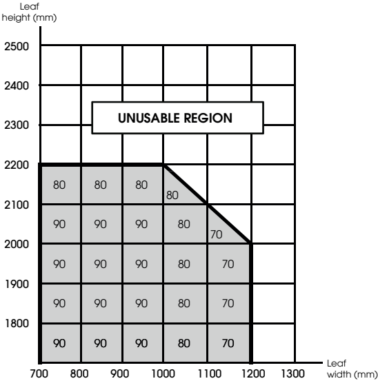
Slot-and-clamp hinge ref 560011 SURFACE-MOUNTING HINGES ref A5081 and A5084
