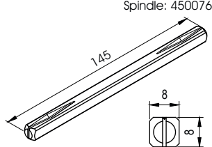
1879 8 mm square spindle for paired lever handles Galvanised steel
