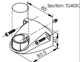
1638 Ø 40 mm tubular handle attachment Powder-coated aluminium
