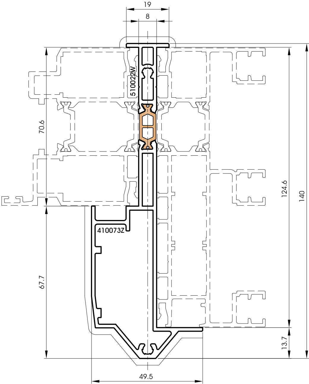
410073 Three-track joint
