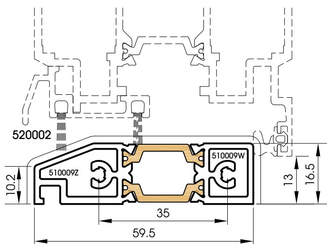
510009 Sill with thermal break
