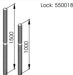
1828 Ø 8 mm locking bar Galvanised steel
