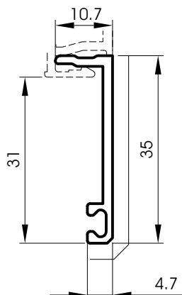
420006 35 mm architrave
