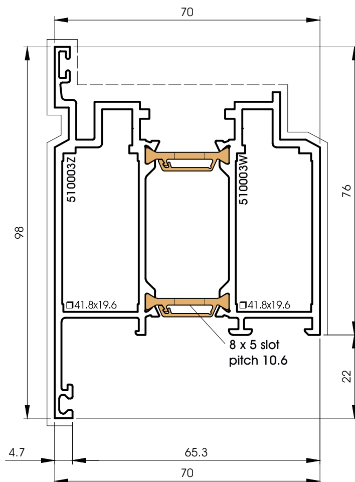
510003 Outward opening
