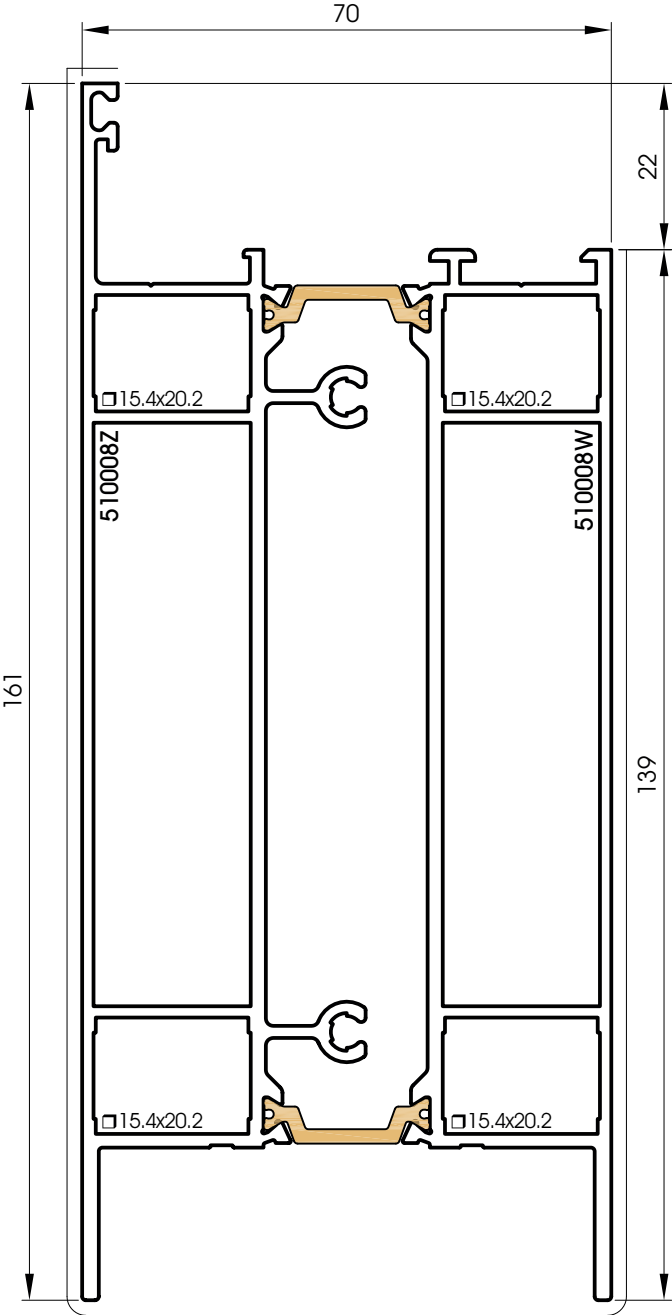
510008 Square-cut kick plate 510008/1 length 1m
