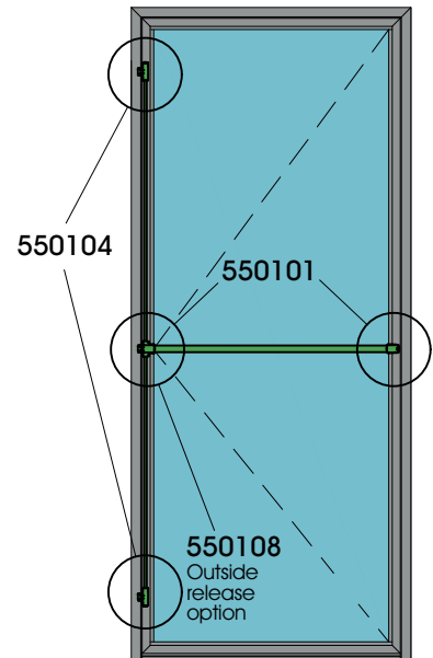
2 or 3 points at side
