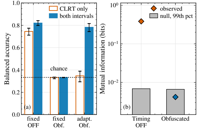
Fig. 8. Transaction-class leakage under the two attacker models, leaving out one grouped run at a time. (a) Balanced accuracy by attacker condition and feature set; whiskers span the 22 held-out runs and are not a confidence interval. (b) Mutual information between the CLRT and the class, against a within-run permutation null.
