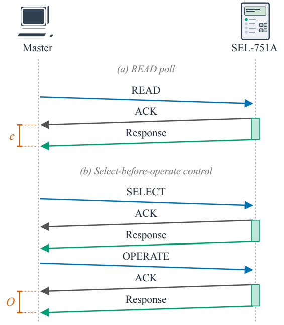
Fig. 1. The two DNP3 transactions we measure, on the master-facing link. (a) A READ poll, whose cross-layer response time runs from the acknowledgment to the response. (b) A select-before-operate control, whose master-visible interval runs from the OPERATE’s acknowledgment to its solicited response. The shaded bar marks the outstation producing the answer; c and O are measured at the master.
