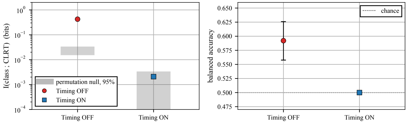
Fig. 7. Timing-only leakage with the timing mechanism disabled and enabled. Left: mutual information between transaction class and CLRT, with the shaded band giving the 95 % permutation null for each arm; with the timing mode off, CLRT carries about 0.42 bits about whether a transaction was a READ or the SELECT phase of an SBO, and with it on the estimate falls inside its own null band, so no dependence remains measurable. Right: balanced accuracy of a classifier trained on Timing OFF CLRT to separate the two classes, applied unchanged to Timing ON traffic, falling from 0.592 to the 0.500 chance baseline. Both panels describe transaction-class feature suppression on a single SEL-751 in a single capture session with a transaction-disjoint, not session-disjoint, split; neither is a device-identification result.
