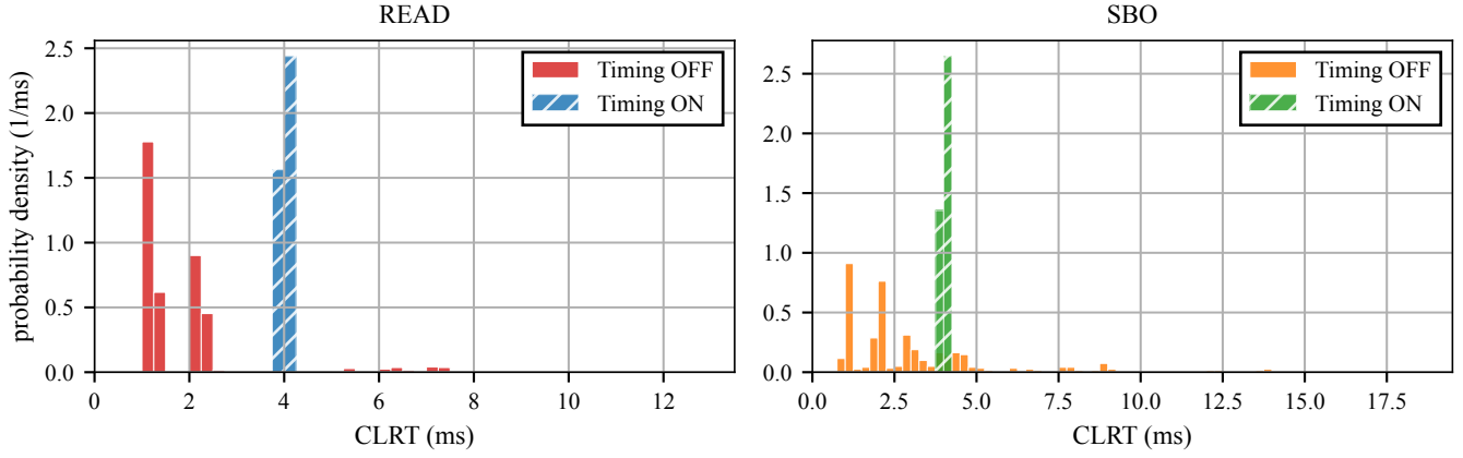
Fig. 4. Cross-layer response time (CLRT), the interval from the outstation's TCP acknowledgment to its DNP3 application response, with the in-network timing mechanism disabled (Timing OFF) and enabled (Timing ON), measured master-facing against the physical SEL-751. Left: READ (function 1). Right: the SELECT phase of select-before-operate (function 3), written SBO throughout; these are SELECT observations, not complete SBO transactions. With the timing mode off, CLRT is spread over roughly 1 to 18 ms and differs between the two classes; with it on, both collapse onto the same 4.001 ms policy value. Timing OFF: 999 READ and 488 SBO transactions; Timing ON: 599 and 499. Each panel's horizontal axis runs to its largest observation, so the full tail is visible. Both arms ran the same unified switch binary with the size-shaping datapath active, so the Timing OFF arm is not an unmodified device baseline and the comparison isolates the timing-mode change.
