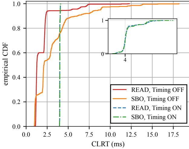
Fig. 5. Empirical CDF of CLRT for READ and for the SELECT phase of SBO, with the timing mechanism disabled (solid) and enabled (dashed). With the timing mode off the two classes separate clearly and the SBO distribution carries a tail to 18.18 ms, shown in full; with it on, both collapse onto 4.001 ms, and the inset magnifies the two Timing ON curves, which coincide at full scale. Size shaping was active in both arms, so Timing OFF is not an unmodified device baseline.
