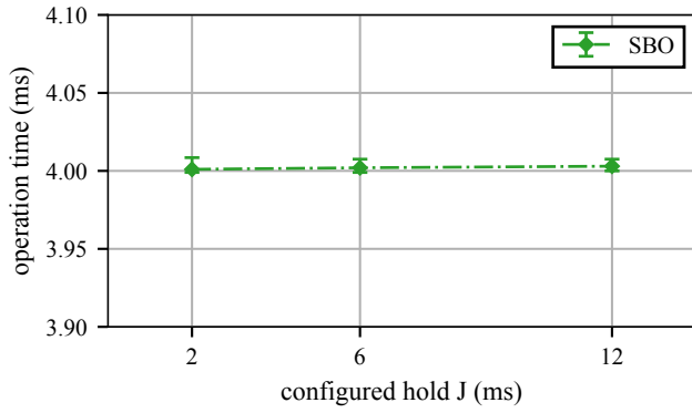
Fig. 8. Master-visible operation time of a select-before-operate control under three configured hold values. The operation time is the interval between the acknowledgment and the echo the master observes, which the design pins to a 4 ms policy value, the same value READ and SBO response times are normalized to in Figures 4 and 5. It stays at that value across J = 2, 6 and 12 ms, so an observer who subtracts the two timestamps available to it learns nothing about the switch-internal hold. Markers are medians of 30 OPERATE transactions per condition; bars are bootstrap 95 % confidence intervals on the median. J is the configured codebook value; it was not observed on the relay-facing wire, and exactly-once relay delivery is not demonstrated.
