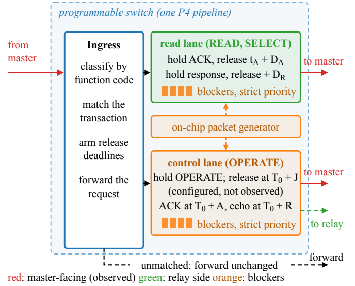
Fig. 3. Design of the hold and timing obfuscation mechanism. Ingress classifies each DNP3 transaction and arms its release deadlines. The read lane holds the acknowledgment and the response of a READ or SELECT and releases them relative to the outstation's acknowledgment. The control lane holds an OPERATE, releases it toward the relay at a configured delay that is not observed, and releases its acknowledgment and solicited response relative to the request. The generator fills the blocker reservoirs (orange); a strict-priority scheduler drains them first, which realizes an armed release deadline when the matching packet arrives within the schedulable window, and otherwise forwards it under the bounded fail-open path so availability is preserved. Red arrows are master-facing and observed; the green dashed arrow is the configured relay-facing release at T_0 + J , not observed. Unmatched traffic is forwarded unchanged.
