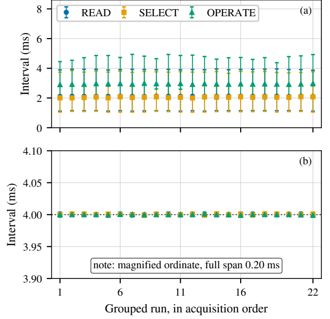
Fig. 7. Within-campaign stability across the 22 grouped runs , in acquisition order. (a) Timing OFF and (b) Obfuscated. Markers are the run median and bars span the interquartile range. Panel (b) uses a magnified ordinate spanning only 0.20 ms around the scheduled release. The 22 runs come from one approximately five-hour campaign on one relay behind one switch and are not independent replications.
