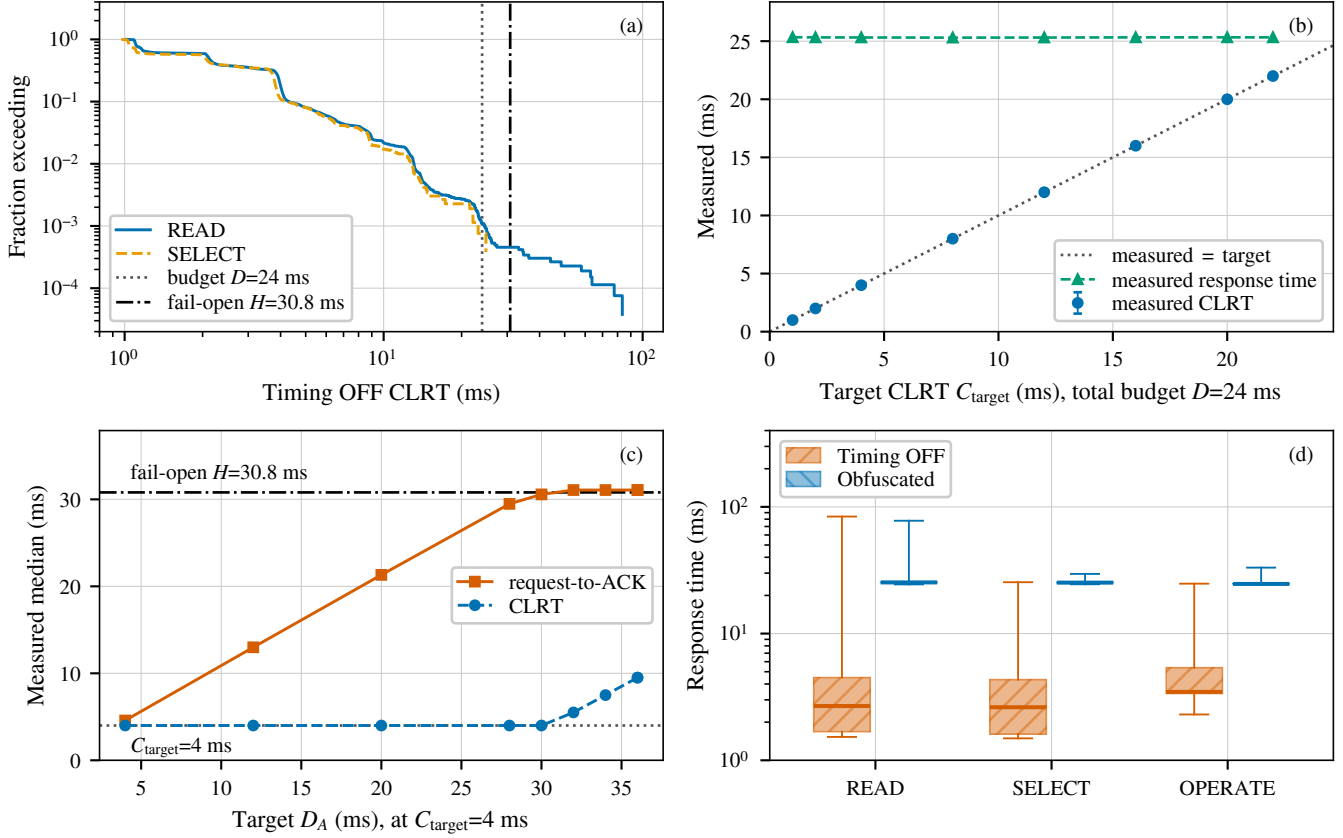
Fig. 8. The release policy is programmable, and its budget is bounded on both sides. (a) Fraction of Timing OFF read-lane exchanges, READ and the SELECT phase of SBO only, whose CLRT exceeds a given value, with the release budget D and the fail-open horizon H . (b) Measured hardware sweep at a fixed total budget D = 24 ms: the visible CLRT follows the configured target along the identity line while the end-to-end response time stays put. (c) Measured sweep of D_A at a fixed target: the request-to-acknowledgment interval tracks the target until it saturates near H , beyond which the CLRT can no longer be held at its target. (d) End-to-end response time per class. Bars in (b) span the interquartile range; boxes in (d) span the quartiles with whiskers over the full support.
