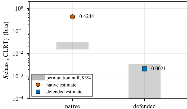
Mutual information
