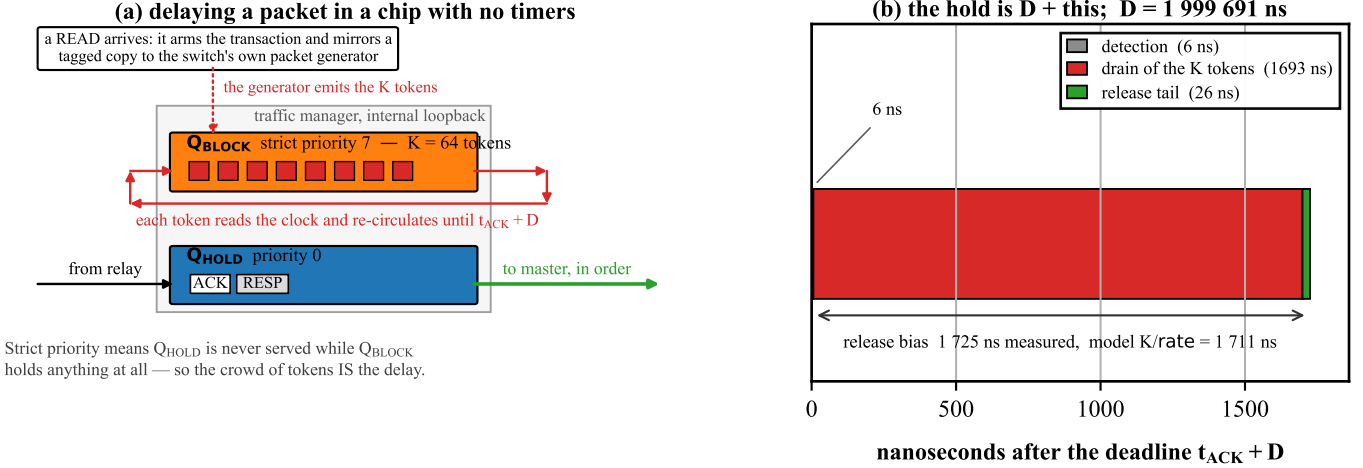
Figure 3: (a) The construction. QBLOCK sits at strict priority 7 and QHOLD at priority 0 on the same internal loopback port, so QHOLD is never served while a single token remains. (b) What happens after the deadline, at nanosecond scale, measured on the physical relay. The hold is D plus these three terms, and D itself is 1 999 691 ns — three orders of magnitude larger, which is why it cannot be drawn on the same axis. Source: figures/src/fig2_mechanism.py.
