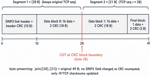
Fig. 3. The 49-byte SEL-751 response and the [28,21] carve. The cut at byte 28 falls on an existing DNP3 CRC-block boundary; the prefix keeps the original TCP sequence number and the suffix advances it by 28, so the master reassembles the identical 49-byte response. No DNP3 byte is modified and no CRC is recomputed.
