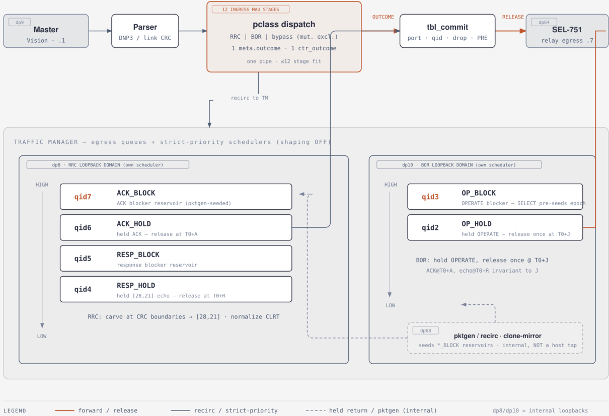
Fig. 2. One-program pipeline and the two scheduling domains. The parser and match-action stages compute a single meta.outcome that a terminal tbl_commit applies. The Traffic Manager holds the RRC reservoirs on dp8 (queues qid7–qid4) and the BOR queue pair on dp10 (qid3,qid2); the packet generator on dp68 seeds the blocker reservoirs. Egress carves the eligible response to [28,21].
