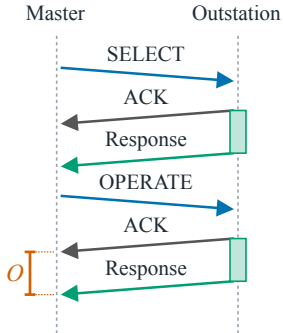
(b) Select-before-operate
