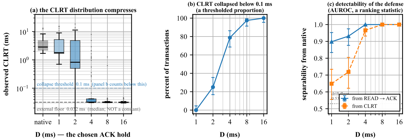
Figure 11: The central result: 480 transactions against the real relay, 400 of them defended. (a) The observed CLRT distribution per arm on a log scale. The distribution compresses onto an external floor of about 0.032 ms — the gray dashed line — as D grows past the relay’s own response time; that floor is the master-capture ACK→RESPONSE gap, not the switch’s 26 ns internal release tail, and it is a tight distribution rather than a constant. (b) The percentage of transactions whose CLRT falls below 0.1 ms — a thresholded sample proportion. (c) How well an adversary separates defended from undefended traffic using each feature — a ranking statistic (AUROC). Error bars are 95 % confidence intervals: a Wilson score interval for the proportion in (b), a bootstrap percentile interval for the AUROC in (c). (b) and (c) are different kinds of quantity and must not be compared arithmetically, so they are separate panels. The dotted line in (c) is the native-versus-native drift floor, 0.53, which is what “no information” looks like in this session. Collapse and detectability rise together, and detection is already near-perfect where the collapse is only partial. Source: figures/src/fig1_dsweep.py.
