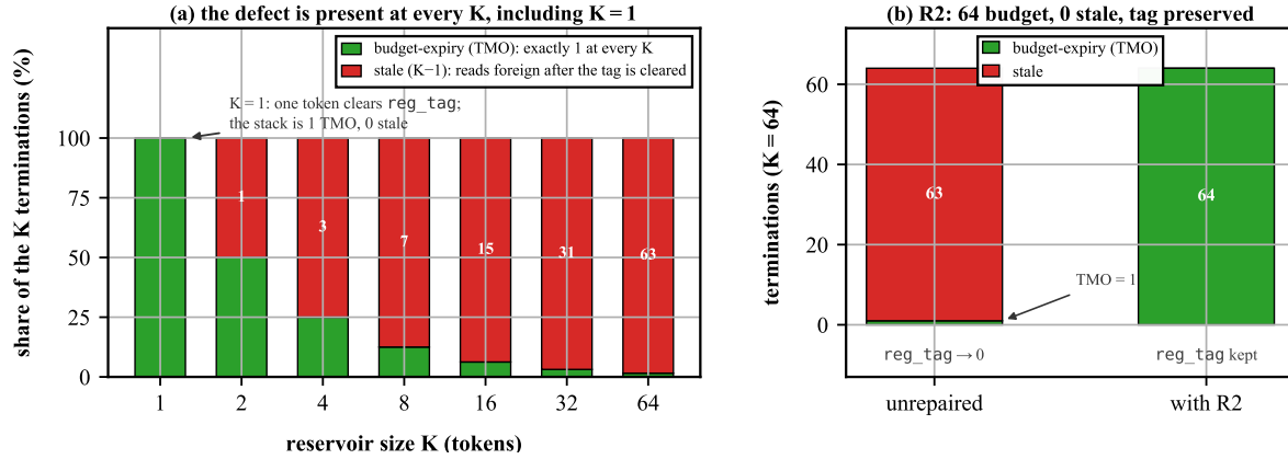
Figure 7: The fail-open reconciliation. (a) On the unrepaired build the budget-zero terminations are 1 (budget) and K - 1 (stale) at every reservoir size, including K = 1 — one native token clears reg_tag and the rest read foreign, so the defect is not an emergent effect of size. (b) R2 turns the same event into K budget terminations and 0 stale, and preserves reg_tag . Source: figures/src/fig9_ksweep.py.
