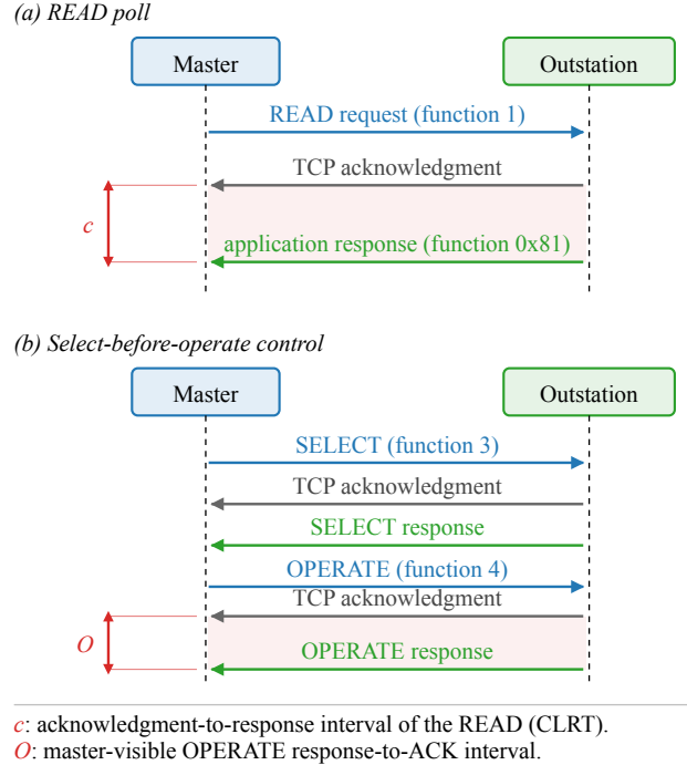
Fig. 1. The two DNP3 transactions we measure, on the master-facing link. (a) A READ poll, whose cross-layer response time c runs from the acknowledgment to the response. (b) A select-before-operate control, whose master-visible interval O runs from the OPERATE’s acknowledgment to its solicited response.
