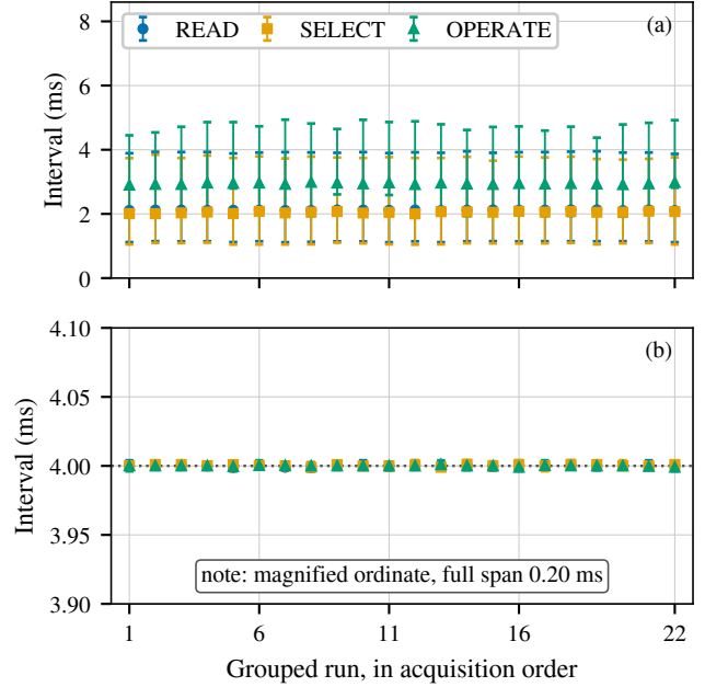
Fig. 7. Per-run medians and interquartile ranges, in acquisition order. Panel (b) uses a magnified ordinate spanning 0.20 ms. The runs are one campaign, not independent replications.
