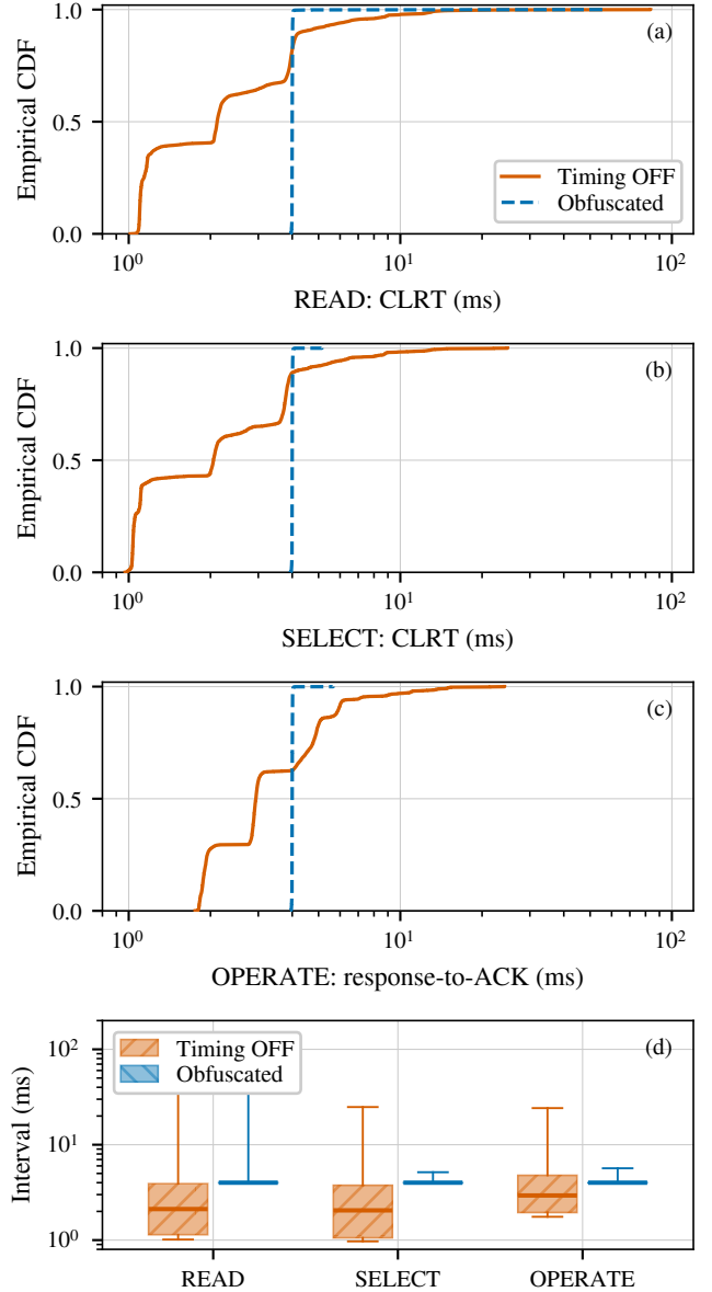
Fig. 6. Measured interval per class. (a) READ and (b) the SELECT phase of SBO report the CLRT; (c) OPERATE reports the master-visible response-to-ACK interval, timed from the request. (d) The same measurements as quartiles. The abscissa is logarithmic and spans the full support.
