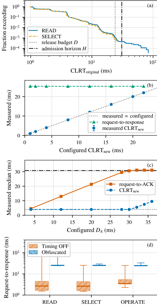
Fig. 9. The release policy is programmable and bounded on both sides. (a) Timing OFF read-lane tail against the budget D and the horizon H . (b) At D = 24 ms the measured \text{CLRT}_{\text{new}} follows the configured \text{CLRT}_{\text{new}} while the response latency stays fixed. (c) Raising D_A saturates near H . (d) End-to-end response time per class.
