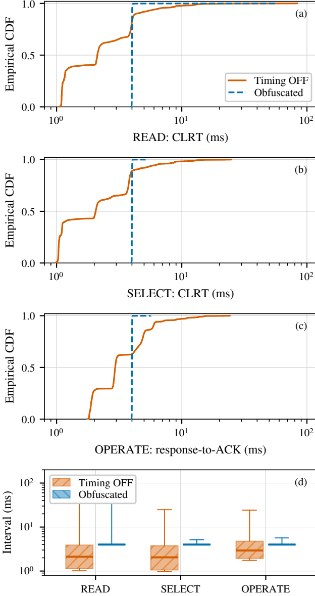
Fig. 7. Measured interval per class. (a) READ and (b) the SELECT phase of SBO report the CLRT; (c) OPERATE reports the master-visible response-to-ACK interval, timed from the request. (d) The same measurements as quartiles. The abscissa is logarithmic and spans the full support.
