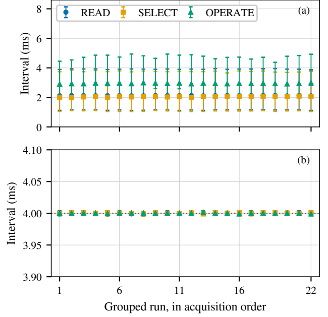
Fig. 8. Per-run medians and interquartile ranges, in acquisition order. Panel (b) uses a magnified ordinate spanning 0.20 ms. The runs are one campaign, not independent replications.
