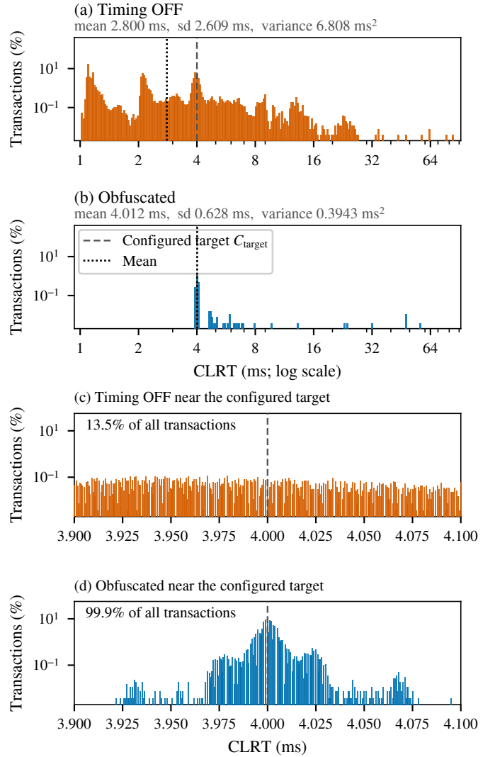
Fig. 5. Measured READ CLRT before and after obfuscation, as a percentage of each arm’s own transactions. (a) and (b) give the full range on logarithmic axes and common bins; (c) and (d) zoom on 0.10 ms either side of the target. The dashed line is the configured target, the dotted line the measured mean.
