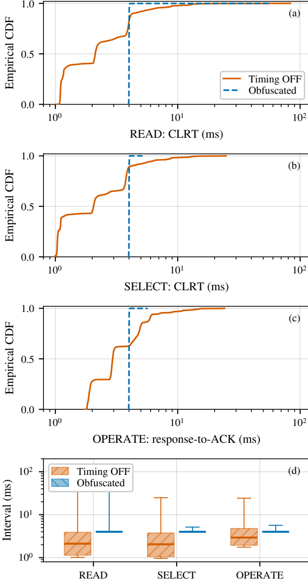
Fig. 6. Measured interval per class over 22 grouped runs. (a) READ and (b) the SELECT phase of SBO report the CLRT; (c) OPERATE reports the master-visible response-to-ACK interval, timed from the request. (d) The same measurements as quartiles. The abscissa is logarithmic and spans the full support.
