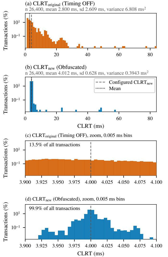
Fig. 5. Measured READ CLRT before and after obfuscation, as a percentage of each arm's own transactions. (a) and (b) give the full range on common 1 ms bins; (c) and (d) repeat the same measurements on 0.005 ms bins within 0.10 ms of the configured \text{CLRT}_{\text{new}} , against the same denominator. Ordinates are logarithmic. The dashed line is the configured value, the dotted line the measured mean.
