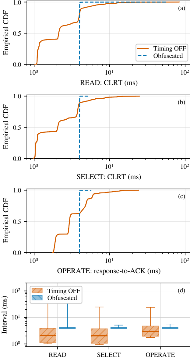
Fig. 6. Measured interval per class. (a) READ and (b) the SELECT phase of SBO report the CLRT; (c) OPERATE reports the master-visible response-to-ACK interval, timed from the request. (d) The same measurements as quartiles. The abscissa is logarithmic and spans the full support.
