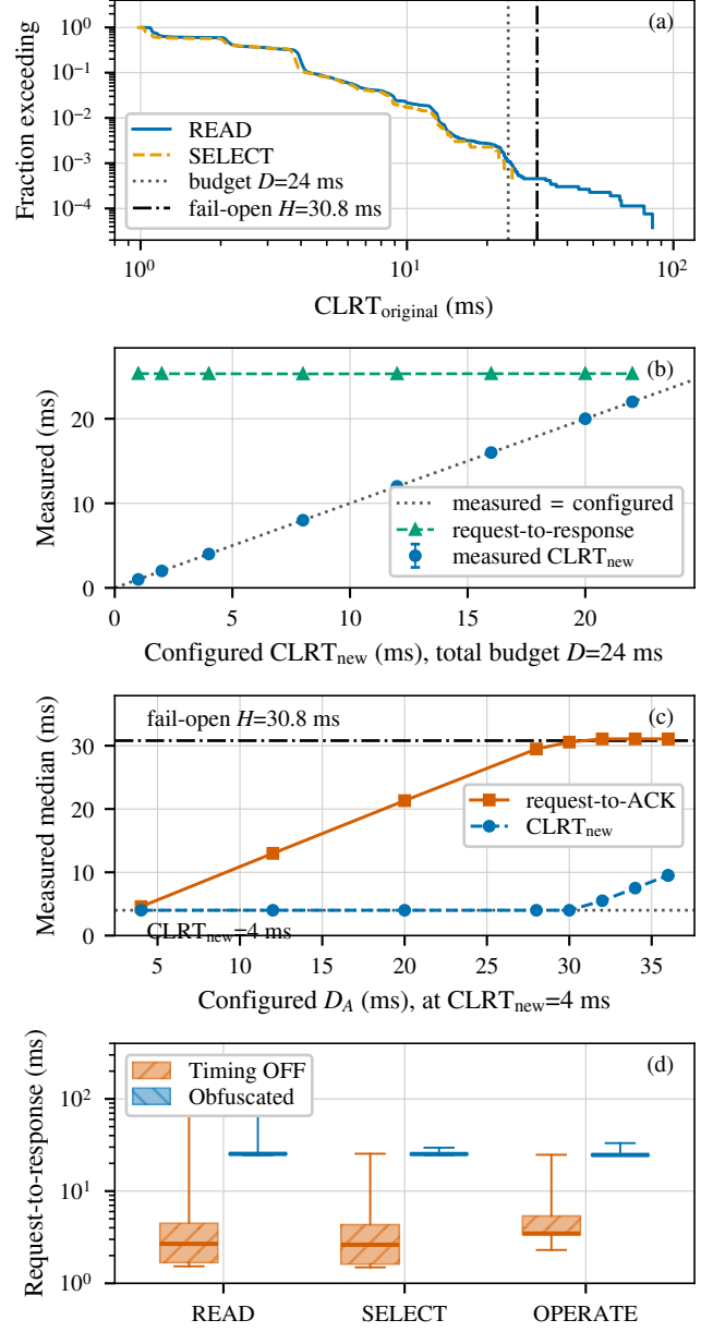
Fig. 8. The release policy is programmable and bounded on both sides. (a) Timing OFF read-lane tail against the budget D and the horizon H . (b) At D = 24 ms the measured \text{CLRT}_{\text{new}} follows the configured \text{CLRT}_{\text{new}} while the response latency stays fixed. (c) Raising D_A saturates near H . (d) End-to-end response time per class.
