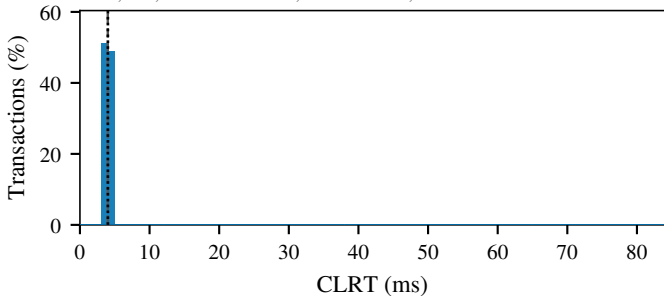
(b) CLRT new (Obfuscated), full range
