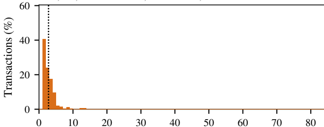
(b) CLRT new (Obfuscated), full range
