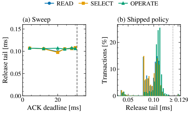
Fig. 8. Release tail \varepsilon . (a) Against the acknowledgment deadline, one series per operation. Past the dashed line the acknowledgment leaves at 31.07 ms whatever the setting, so the deadline is not met and no tail is defined. (b) Its distribution at the campaign policy; the rightmost category includes every tail at or above 0.129 ms. Percentages use each operation’s entire sample as the denominator.
