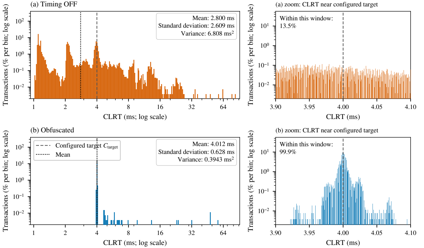
Fig. 5. Measured READ CLRT before and after obfuscation. (a) Timing OFF and (b) Obfuscated, over the 22 grouped runs. Left: the full measured range on logarithmic axes, on common bin edges spaced evenly in \log_{10} and identical limits, so a bar in (a) and a bar in (b) mean the same at the same height. Right: a linear zoom on a 0.10 ms window either side of the configured target. Bars are the percentage of that arm’s own transactions in each bin, so the comparison does not depend on sample size; in the zoom the denominator is still the arm’s full sample, and the share falling inside the window is stated on the panel. The dashed line is the configured target C_{\text{target}} , a policy value and not a measurement; the dotted line is the measured mean. Nothing is smoothed and no tail is clipped.
