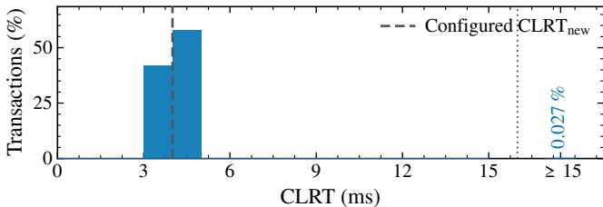
(b) Obfuscated
