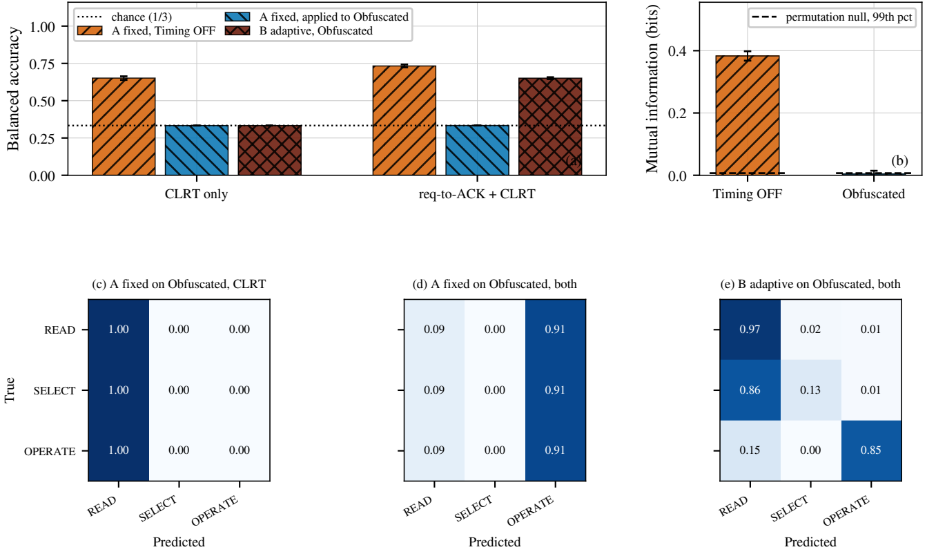
Fig. 8. Transaction-class leakage under the two attacker models , leaving out one grouped run at a time over all 22 runs. (a) Balanced accuracy with grouped-run 95% confidence intervals. (b) Mutual information in bits with jackknife intervals and the 99th percentile of a within-run permutation null. (c) to (e) Row-normalised confusion over all 22 held-out runs.
