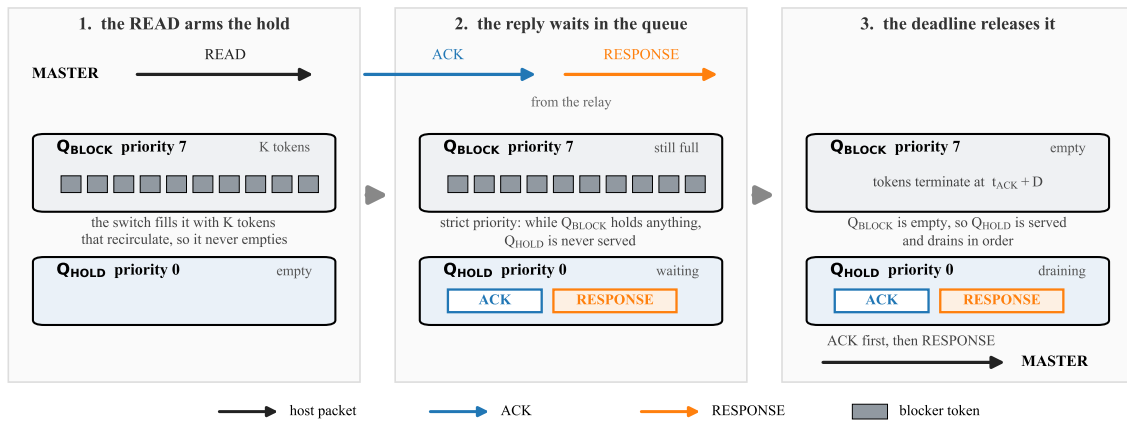
Figure 8: The mechanism, in three stages, read left to right. 1 A READ arms the transaction and the switch fills Q\_BLOCK (strict priority 7) with K self-recirculating tokens, so that queue never empties. 2 The relay’s ACK and its RESPONSE land in Q\_HOLD (priority 0); strict priority means Q\_HOLD is not served while Q\_BLOCK holds anything at all, so the crowd of tokens is the delay. 3 At the deadline t_{ACK} + D the tokens terminate, Q\_BLOCK empties, and Q\_HOLD drains in order — the ACK first, then the RESPONSE. The figure is deliberately mechanism-only: the three repairs and the parser/sequence fixes are the subject of §8 and are not drawn here.
