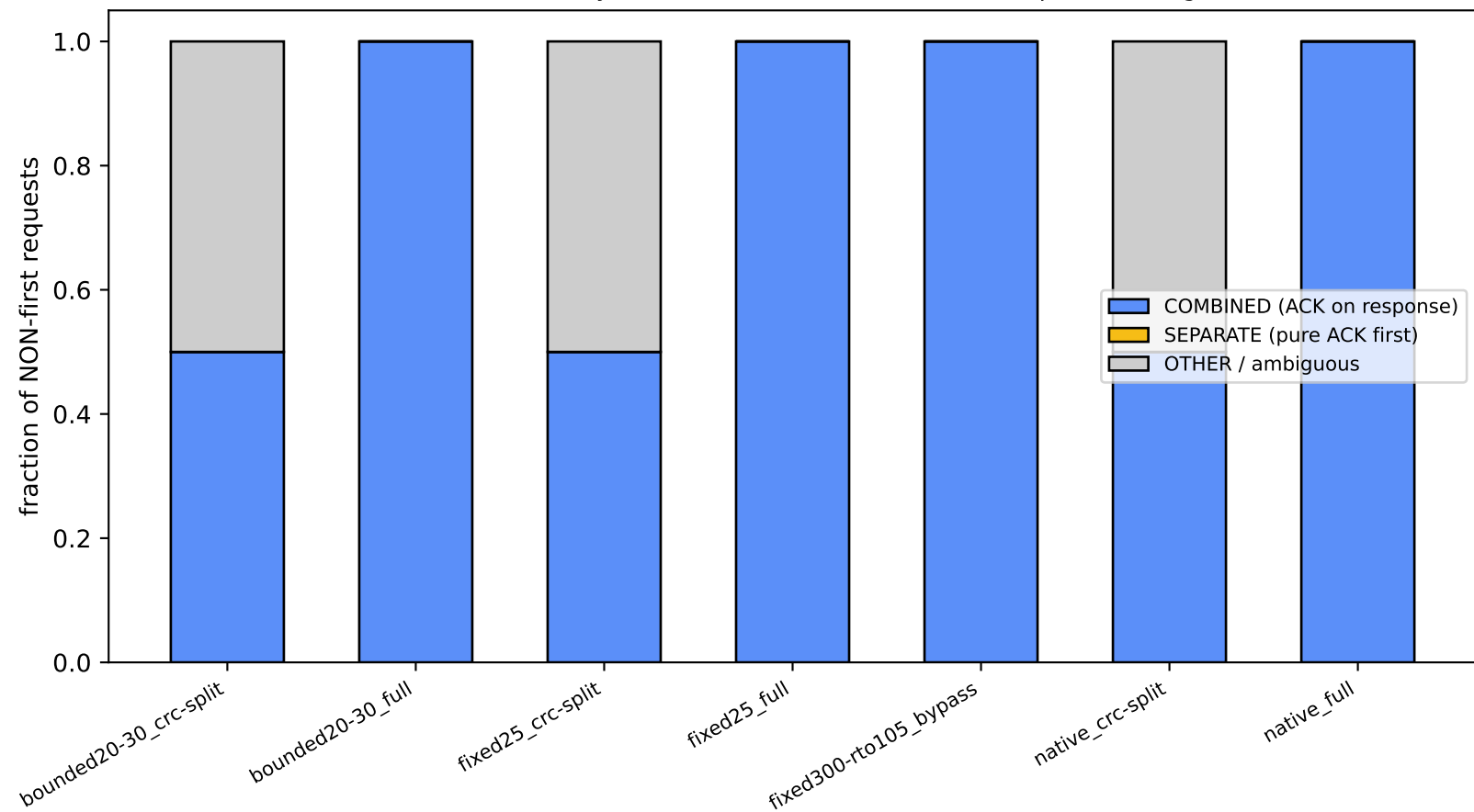
Phase 03A: ACK mode by config (non-first requests) fixed25 / bounded20-30 stay 100% COMBINED like native; crc-split chunking -> OTHER
