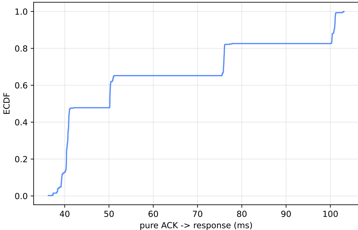
Phase 03A: pure-ACK->response CDF (separated non-first) gap tracks the configured application-write delay (36-100 ms across sampled delays)
