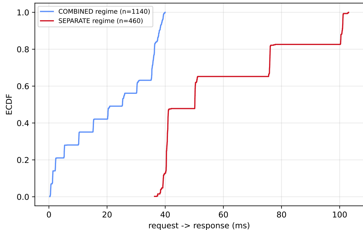
Phase 03A: request->response CDF by ACK regime (non-first)
