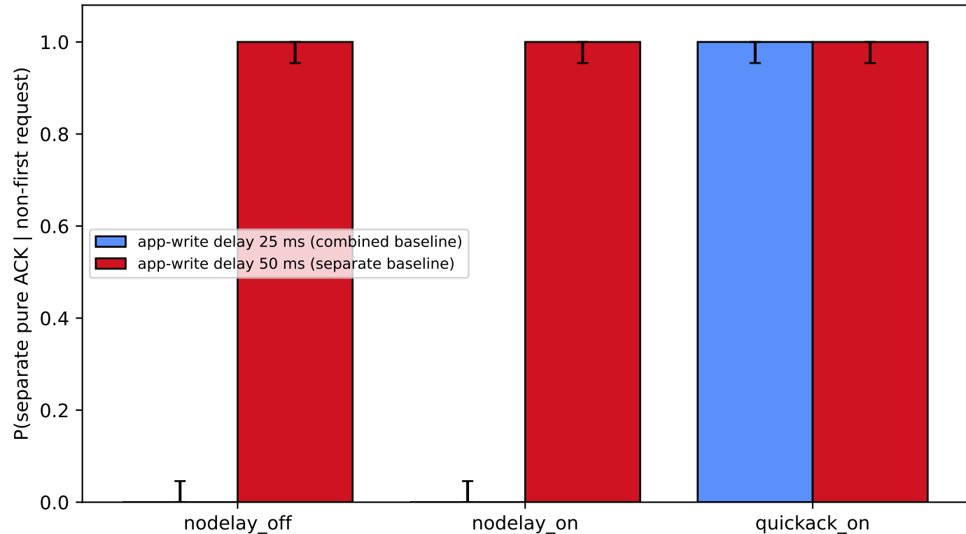
Phase 03A: socket-option effect on ACK separation (RQ3) one factor at a time; Wilson 95% CIs
