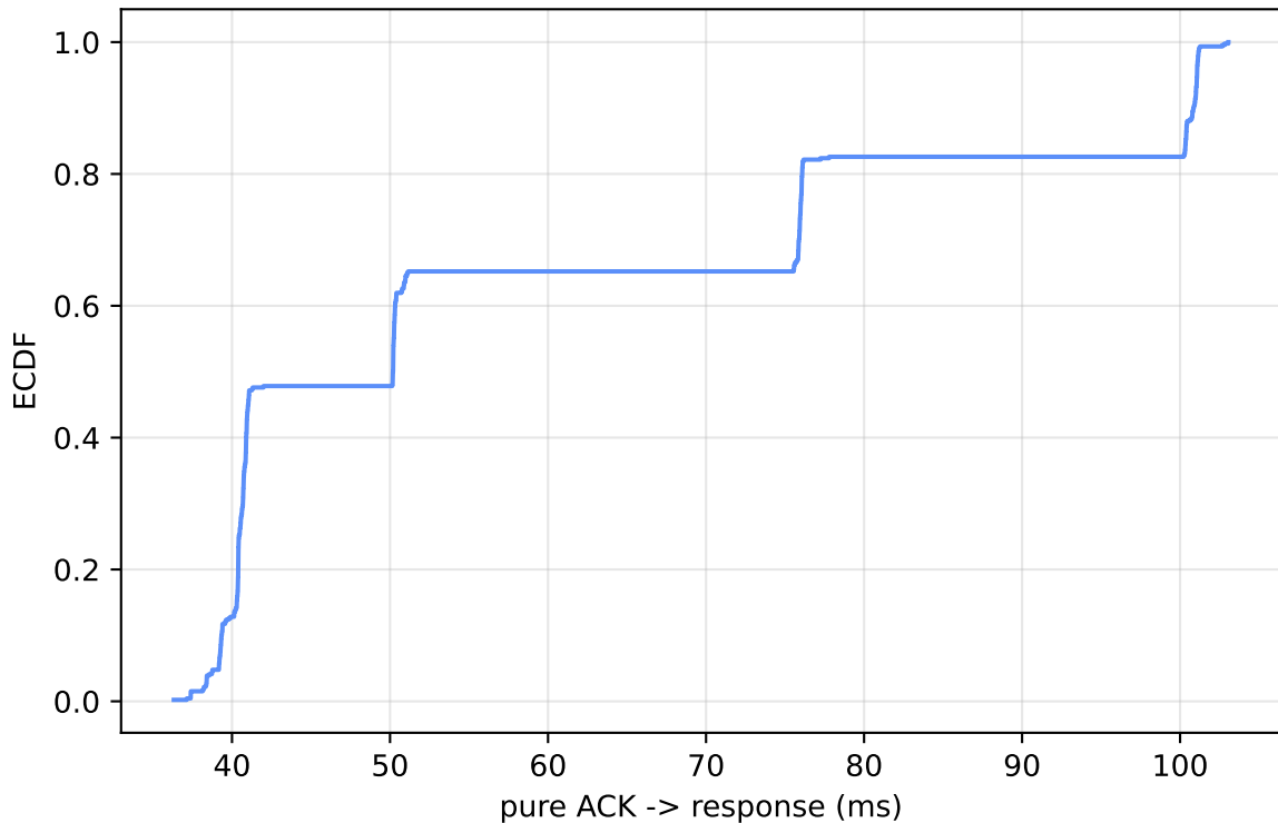
Phase 03A: pure-ACK->response CDF (separated non-first) gap tracks the configured application-write delay ( \geq \sim 40 ms here)
