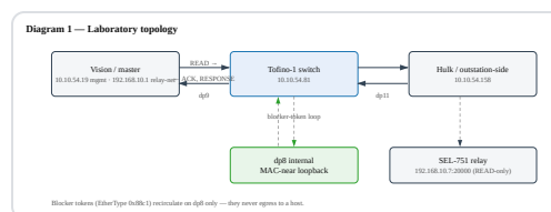
Diagram 1 — the lab: master (Vision), Tofino-1 switch, outstation-side host (Hulk), and the physical SEL-751 relay. dp8 is an internal loopback used only inside the switch.
