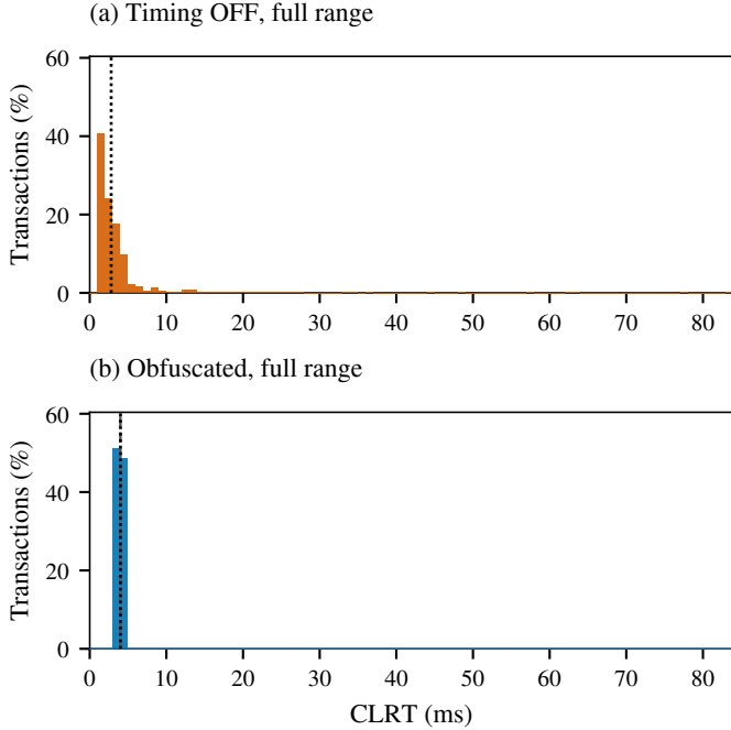
Fig. 7. The same measurements over the entire measured range. Identical 1 ms bins anchored at 0 ms and no overflow category, so every tail out to the largest observation, 83.5 ms in (a) and 57.2 ms in (b), is drawn. This is the companion to Figure 5, which truncates at 15 ms to keep the body of the distributions legible.
