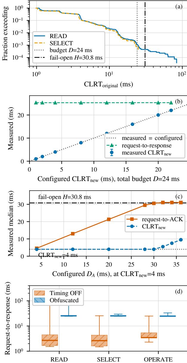
Fig. 10. The release policy is programmable and bounded on both sides. (a) Timing OFF read-lane tail against the budget D and the horizon H . (b) At D = 24 ms the measured CLRT_{new} follows the configured CLRT_{new} while the response latency stays fixed. (c) Raising D_A saturates near H . (d) End-to-end response time per class.
