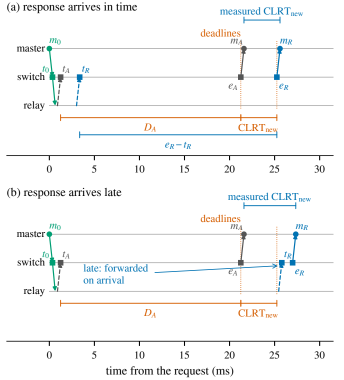
Fig. 3. Release timeline of one READ transaction. Both deadlines are computed from the acknowledgment's arrival t_A . In (a) the response arrives in time and the master observes the configured \text{CLRT}_{\text{new}} ; in (b) it arrives late and the switch forwards it at once. The response hold e_R - t_R is drawn in (a) because it is implied by the schedule, not configured. Filled circles were measured, open squares were not.
