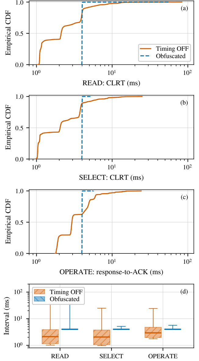
Fig. 8. Measured interval per class. (a) READ and (b) the SELECT phase of SBO report the CLRT; (c) OPERATE reports the master-visible response-to-ACK interval, timed from the request. (d) The same measurements as quartiles. The abscissa is logarithmic and spans the full support.
