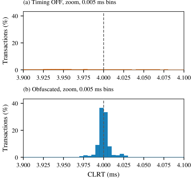
Fig. 6. The released interval, resolved. The same measurements as Figure 5 on 0.005 ms bins within 0.10 ms of the configured CLRT_{new} (dashed). The ordinate is still the percentage of that arm's entire sample, not of the window, so the bars are directly comparable with the other figures. The window holds 13.53% of (a) and 99.86% of (b).
