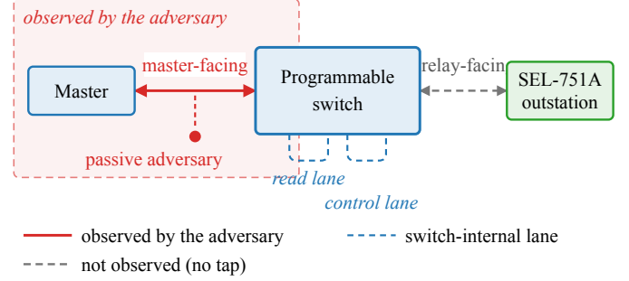
Fig. 2. Observation model. The master reaches the SEL-751A outstation through one programmable switch. The passive adversary sees only the master-facing link (solid red, shaded region); the relay-facing link and the two switch-internal scheduling lanes (dashed) are not observed, by the adversary or by our measurements.
