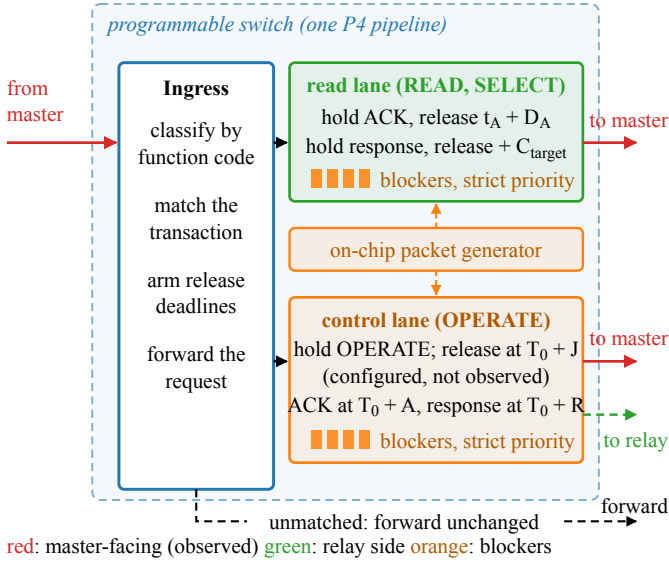
Fig. 4. How one pipeline realizes the schedule. Ingress classifies each DNP3 transaction and arms its release deadlines. The read lane holds the acknowledgment and the response of a READ or SELECT and releases them relative to the outstation's acknowledgment; the control lane holds an OPERATE, releases it toward the relay at a configured delay that we do not observe, and releases the acknowledgment and solicited response relative to the request. The packet generator fills the blocker reservoirs (orange), and a strict-priority scheduler drains them before the held packet, which is what sustains a hold until its deadline expires. Red arrows are master-facing and observed; the green dashed arrow is the configured relay-facing release, which is not. Unmatched traffic is forwarded unchanged.
