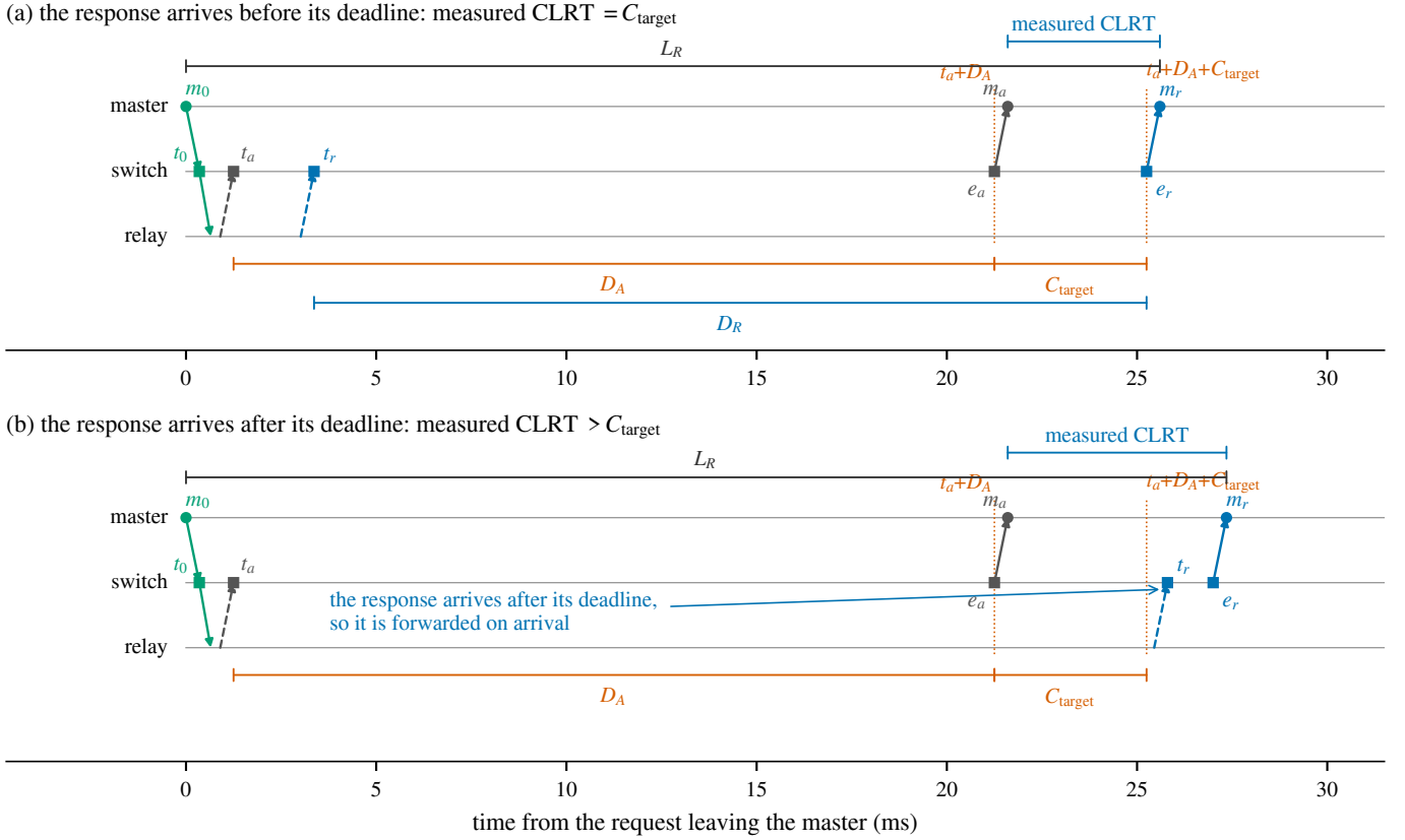
Fig. 3. Release timeline of one READ transaction. The switch arms both deadlines from a single anchor, the arrival of the outstation's acknowledgment at t_a . In (a) the response arrives before its deadline, so the master observes the configured target. In (b) it arrives after, and the switch forwards it on arrival. The response hold D_R is drawn in (a) to show that it is not a configured constant: it is whatever the schedule requires, so it moves with the arrival t_r . Only m_0 , m_a and m_r were measured; the four switch-side instants were not. Propagation and the switch's processing term are drawn at a legible size, not to scale.
