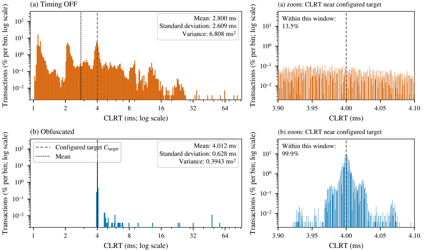
Fig. 6. Measured READ CLRT before and after obfuscation. (a) Timing OFF and (b) Obfuscated, over the 22 grouped runs. Left: the full measured range on logarithmic axes, on common bin edges spaced evenly in \log_{10} and identical limits, so a bar in (a) and a bar in (b) mean the same at the same height. Right: a linear zoom on a 0.10 ms window either side of the configured target. Bars are the percentage of that arm’s own transactions in each bin, so the comparison does not depend on sample size; in the zoom the denominator is still the arm’s full sample, and the share falling inside the window is stated on the panel. The dashed line is the configured target C_{\text{target}} , a policy value and not a measurement; the dotted line is the measured mean. Nothing is smoothed and no tail is clipped.
