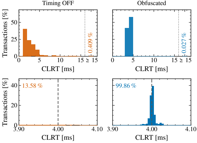
Fig. 5. READ CLRT measured on the master-facing link, in both cases (columns) and at two scales (rows). The upper row uses 1 ms bins, and its last bin holds every interval of 15 ms or more. The lower row uses 0.005 ms bins within 0.10 ms of the configured \text{CLRT}_{\text{new}} (dashed). Both rows give the percentage of all 26,400 exchanges of each case.
