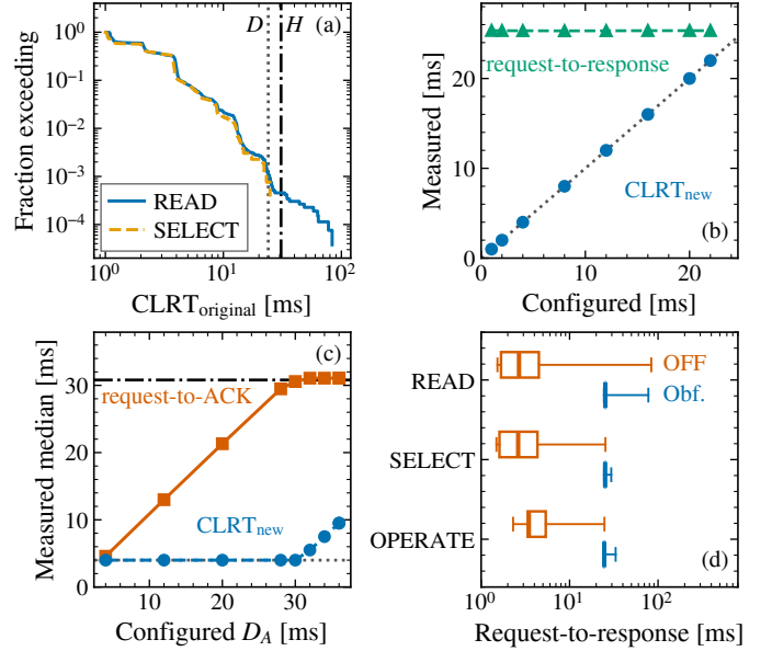
Fig. 6. Release policy and cost. (a) Timing OFF response time of the read lane against the budget D and the horizon H . (b) At D = 24 ms, the measured \text{CLRT}_{\text{new}} against the configured one, with the response time of the exchange. (c) The measured request-to-acknowledgment interval against the configured D_A . (d) End-to-end response time per class in both cases.
