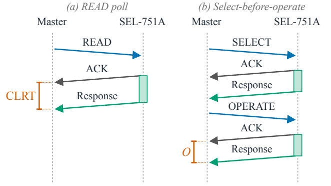
Fig. 1. The two DNP3 transactions, observed on the master-facing link. (a) A READ poll, whose CLRT runs from the acknowledgment to the response. (b) A select-before-operate control, whose master-visible interval O runs from the acknowledgment of the OPERATE to its response. The shaded bar marks the outstation producing the answer.
