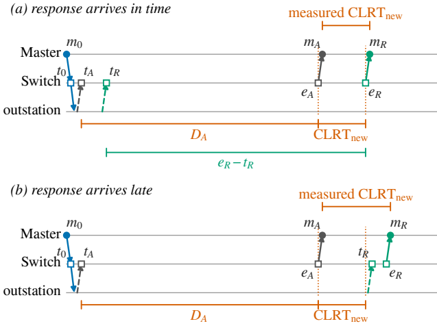
Fig. 4. Release timeline of one READ transaction. The drawing is schematic and its spacing is not to scale. Both deadlines are computed from the arrival of the acknowledgment t_A . In (a), the response arrives in time and the master observes the configured \text{CLRT}_{\text{new}} . In (b), it arrives late and leaves when its queue serves it. Filled circles lie on the master-facing link. Open squares are instants inside the switch.
