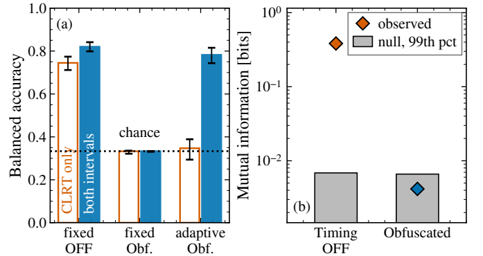
Fig. 7. Fingerprinting the three operations, with one grouped run held out at a time. (a) Balanced accuracy of a fixed adversary tested on Timing OFF and on Obfuscated traffic, and of an adaptive adversary retrained on Obfuscated traffic. Whiskers span the 22 held-out runs. (b) Mutual information between the CLRT and the operation, against a within-run permutation null.
