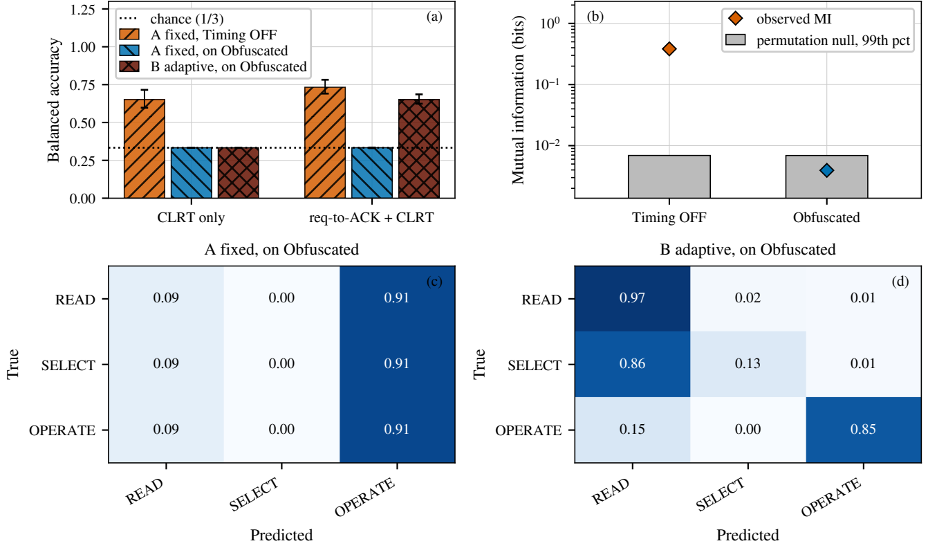
Fig. 8. Transaction-class leakage under the two attacker models , leaving out one grouped run at a time over all 22 runs. (a) Balanced accuracy of the evaluated Random-Forest attacker; bars are the mean over the 22 held-out runs and the whiskers span the full range across those runs, which is within-campaign variability and not a confidence interval, because the folds share training data. (b) Observed mutual information between the CLRT and the transaction class against the 99th percentile of a within-run permutation null. (c) and (d) Row-normalised confusion over all 22 held-out runs, using both intervals.
