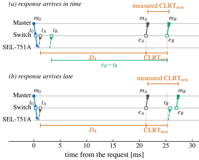
Fig. 3. Release timeline of one READ transaction. Time coordinates are illustrative, chosen so an arrival and its emission are separable on the page. Both deadlines are computed from the acknowledgment's arrival t_A : in (a) the response arrives in time and the master observes the configured \text{CLRT}_{\text{new}} , in (b) it arrives late. The response hold e_R - t_R is drawn in (a) because the schedule implies it rather than configuring it. Filled circles lie on the master-facing link, the only place this work captured anything; open squares are switch-side instants that were not captured.
