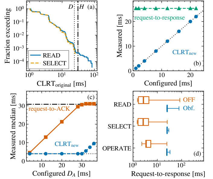
Fig. 6. The release policy is programmable and bounded on both sides. (a) Timing OFF read-lane tail against the budget D and the horizon H . (b) At D = 24 ms the measured \text{CLRT}_{\text{new}} follows the configured \text{CLRT}_{\text{new}} while the response latency stays fixed. (c) Raising D_A saturates near H . (d) End-to-end response time per class.
