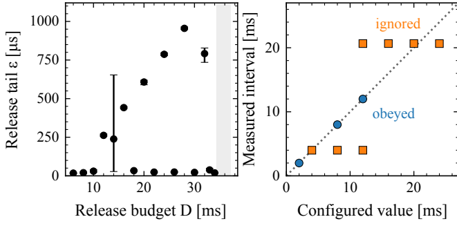
Fig. 7. (a) The release tail \epsilon against the budget D , over three installs of each setting; whiskers span them. In the shaded region the reservoir spends its pass budget and releases early, so no tail is defined. (b) Each configured quantity that could set a master-visible OPERATE interval, against the interval it would set: the configured \text{CLRT}_{\text{new}} is obeyed, and the control plane’s offsets A and R - A are ignored.
