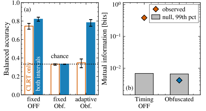
Fig. 8. Transaction-class leakage under the two attacker models, leaving out one grouped run at a time. (a) Balanced accuracy by attacker condition and feature set. The abscissa names the training condition and the arm it is tested on: fixed on Timing OFF, the same fixed model on Obfuscated traffic, and a model retrained on Obfuscated traffic. Whiskers span the 22 held-out runs and are not a confidence interval. (b) Mutual information between the CLRT and the class, against a within-run permutation null.
